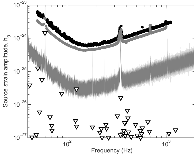
Figure 13. Limits on GW strain from rotating neutron stars. Upper curve (black points): all-sky strain upper limits on unknown neutron stars for spindown rates as high as 5 \times 10^{-9} \text{ Hz s}^{-1} and optimal orientation, from analysis of the first 8 months of S5 data [89]. Middle curve (gray points): expected sensitivity for the Einstein@Home search with 5280 hrs of S5 data. Lower curve (gray band): expected range for 95% confidence level Bayesian upper limits on radio pulsars with known ephemerides, using the full S5 data. Black triangles: upper limits on GW emission from known radio pulsars based on their observed spin-down rates.
