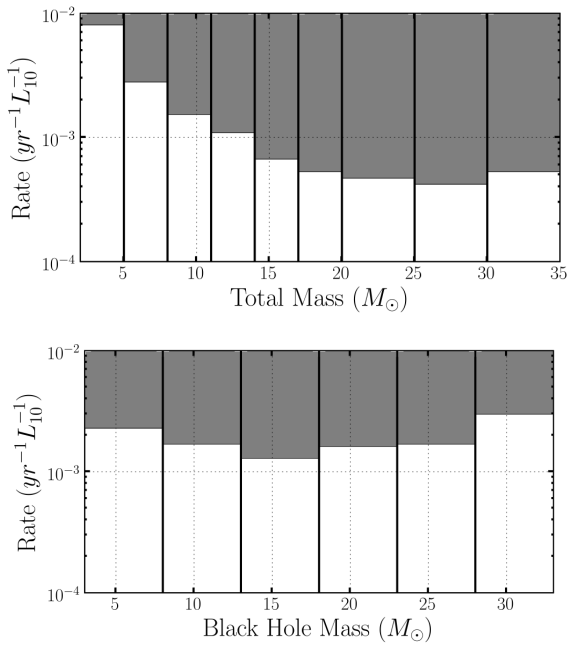
FIG. 2: The marginalized 90% rate upper limits as a function of mass. The upper plot shows limits for BBH systems as a function of the total mass of the system. The lower plot shows limits for BHNS systems as a function of the black hole mass, assuming a fixed neutron star mass of 1.35M_{\odot} . Here the upper limits are calculated using only H1H2L1 data since the relatively small amount of H1L1 and H2L1 data makes it difficult to evaluate the cumulative luminosity in the individual mass bins.
