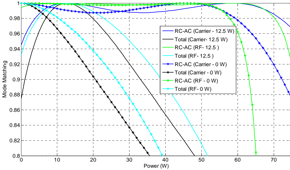
Fig. 3: Coupling between various modes for both carrier and the RF sidebands. Here RC-AC represents the coupling between the arm cavity mode and the recycling cavity mode. Total represents the product of coupling between AC-RC and IMC-RC.
