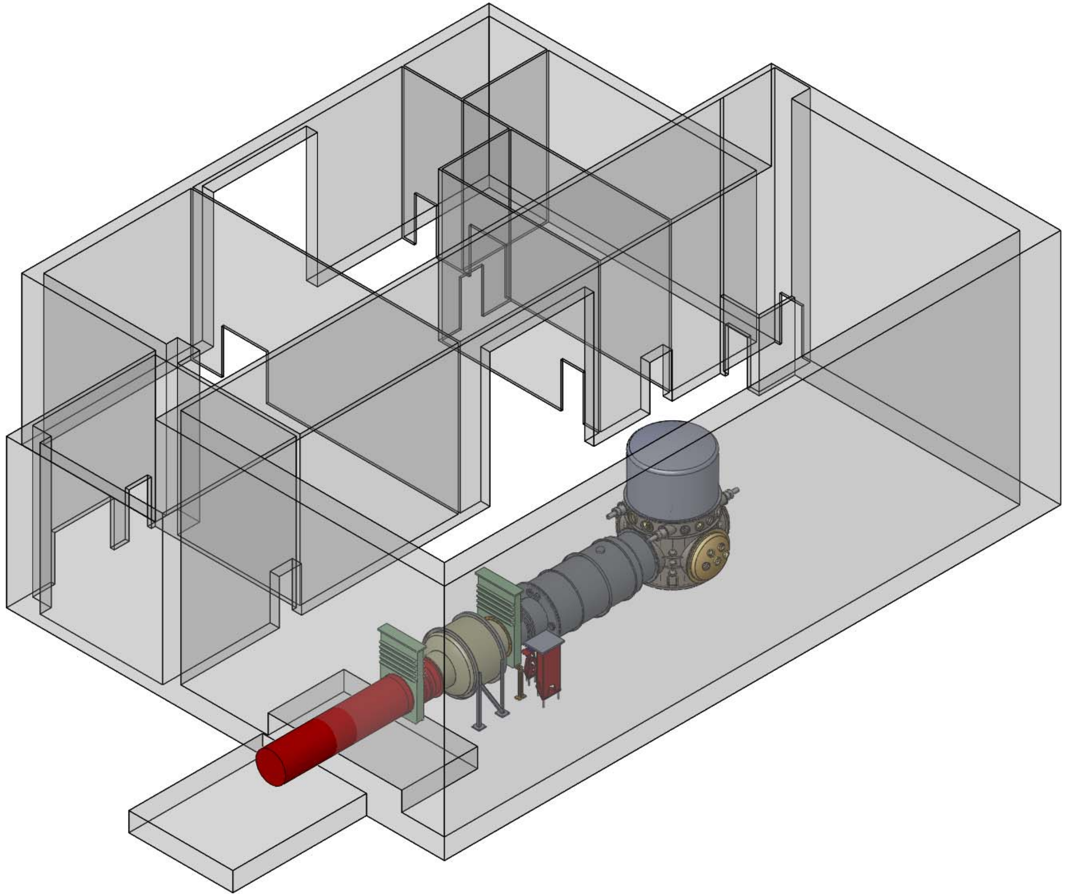
D0901464 AdvLIGO Systems Layout LLO Y-End Station (ISO View)
