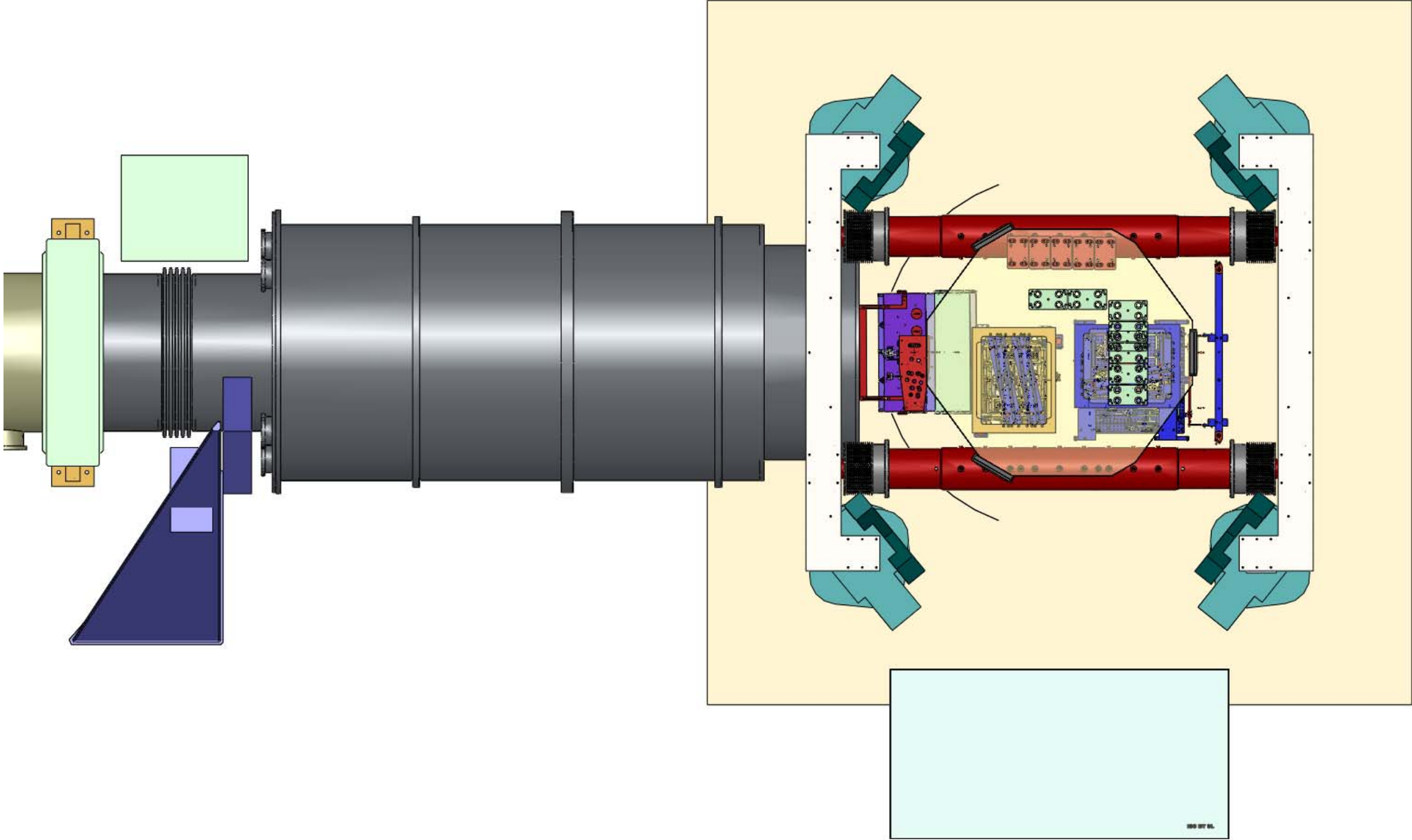
D0901465 AdvLIGO Systems Layout LLO X-End Station (BSC4 View)
