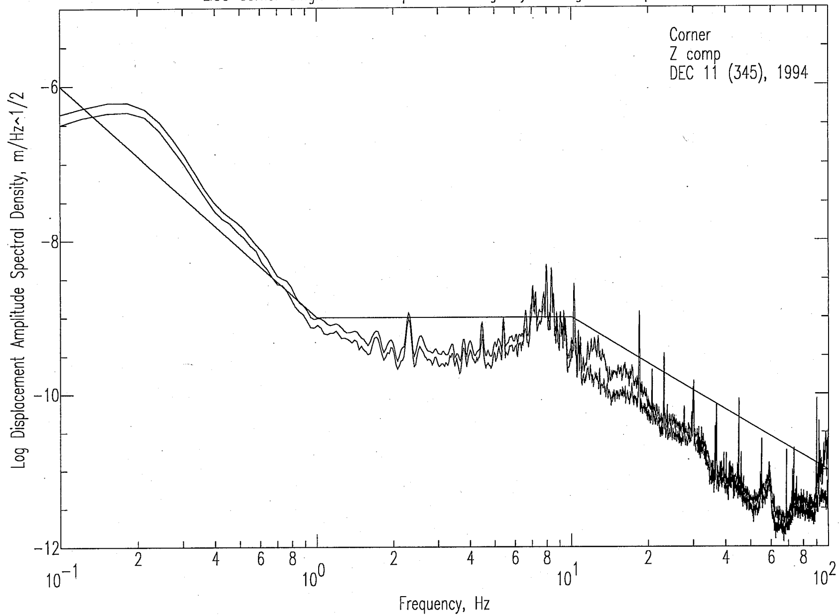
LIGO Corner Single Vehicle 3 passes on Highway 10 seg3.1.sac Spectra
