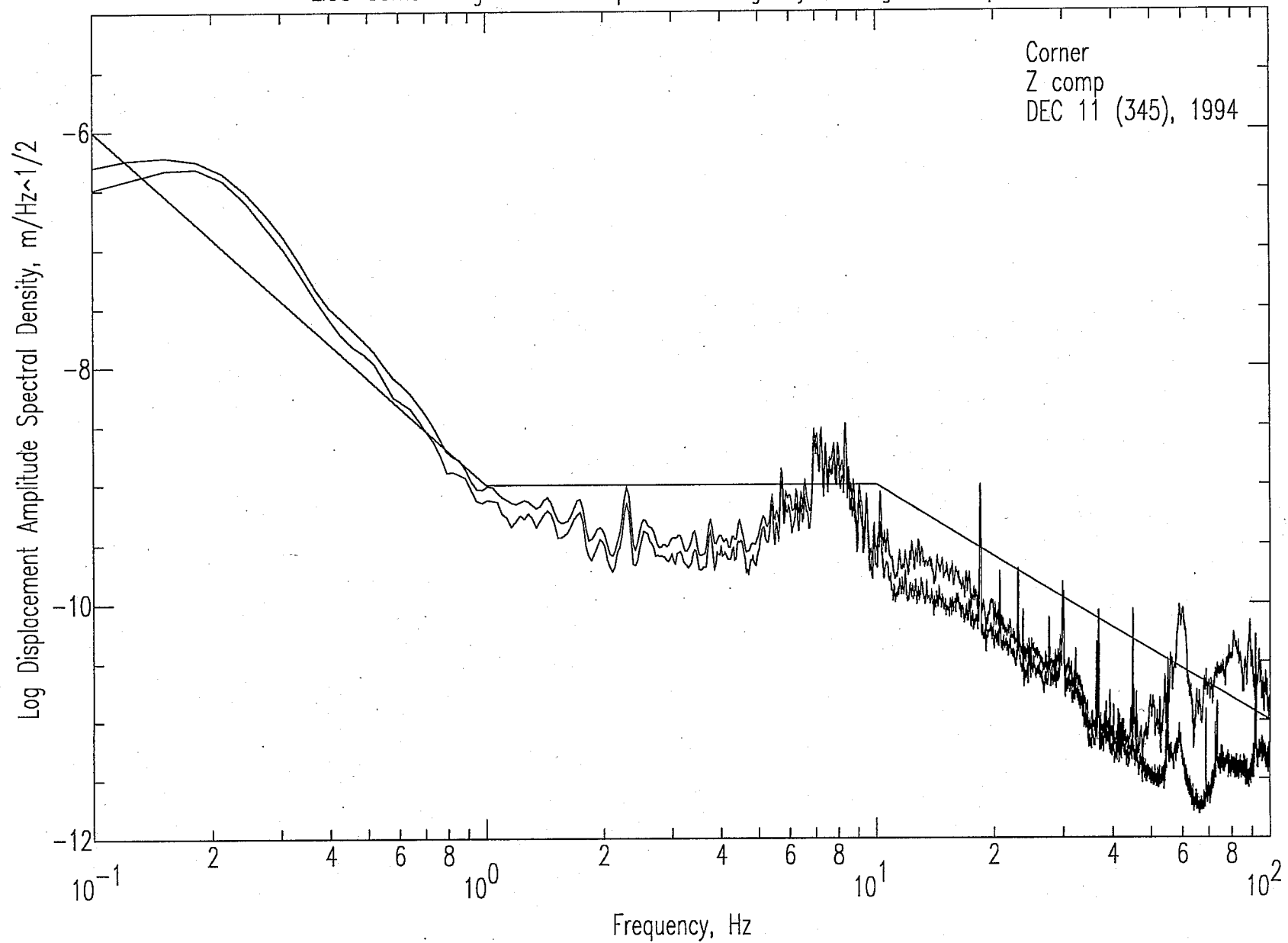
LIGO Corner Single Vehicle 3 passes on Highway 10 seg2.1.sac Spectra
