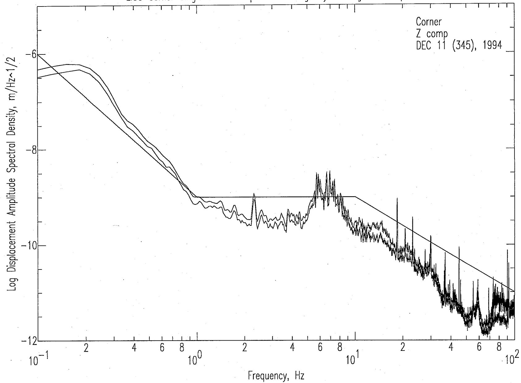
LIGO Corner Single Vehicle 3 passes on Highway 10 seg1.1.sac Spectra
