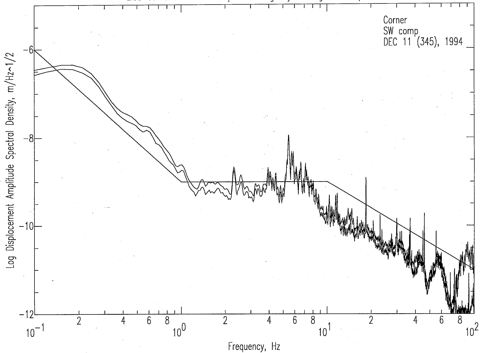
LIGO Corner Patrol car 1 pass on Highway 10 seg0.3.sac Spectra
