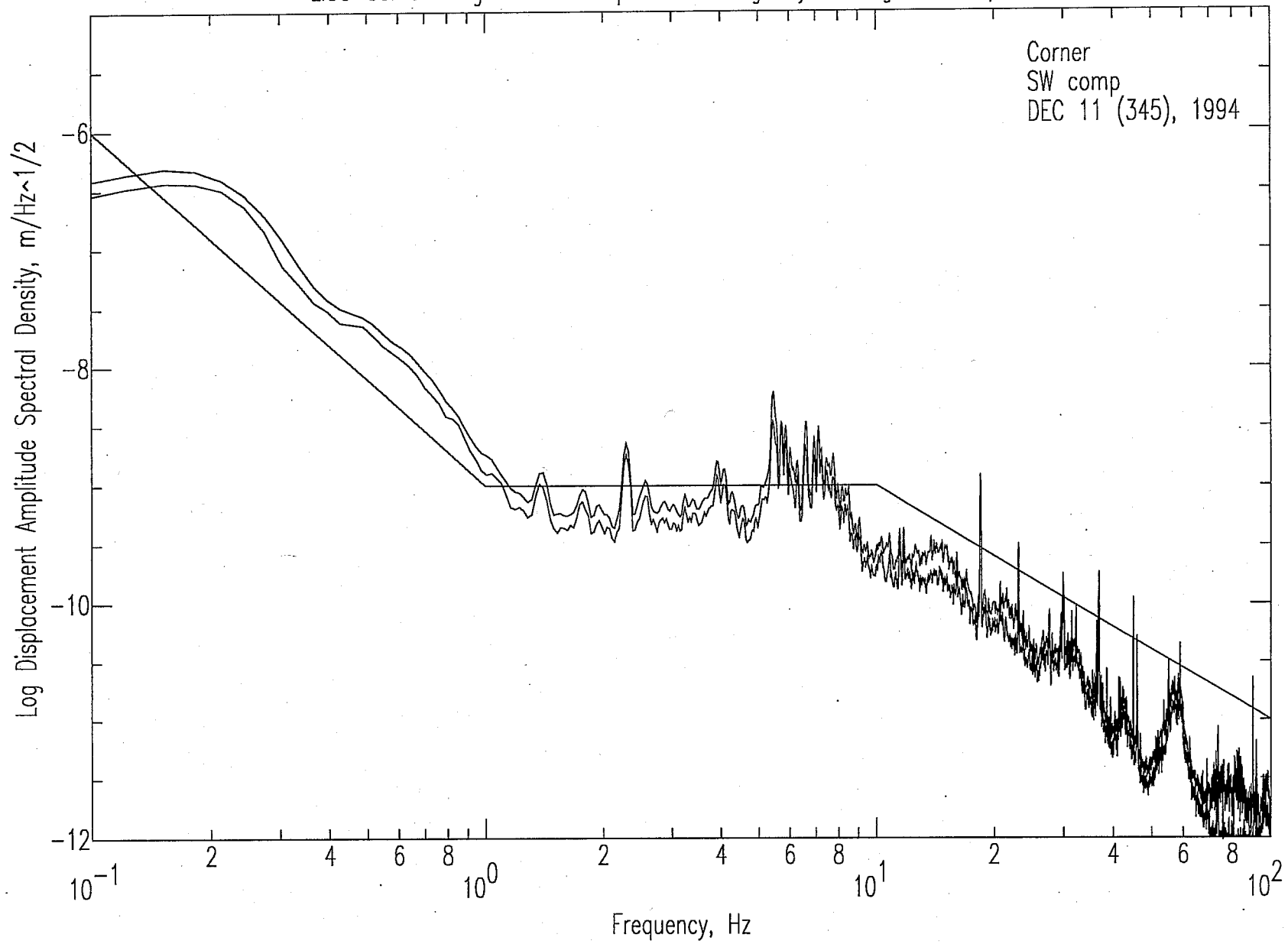
LIGO Corner Single Vehicle 3 passes on Highway 10 seg1.3.sac Spectra
