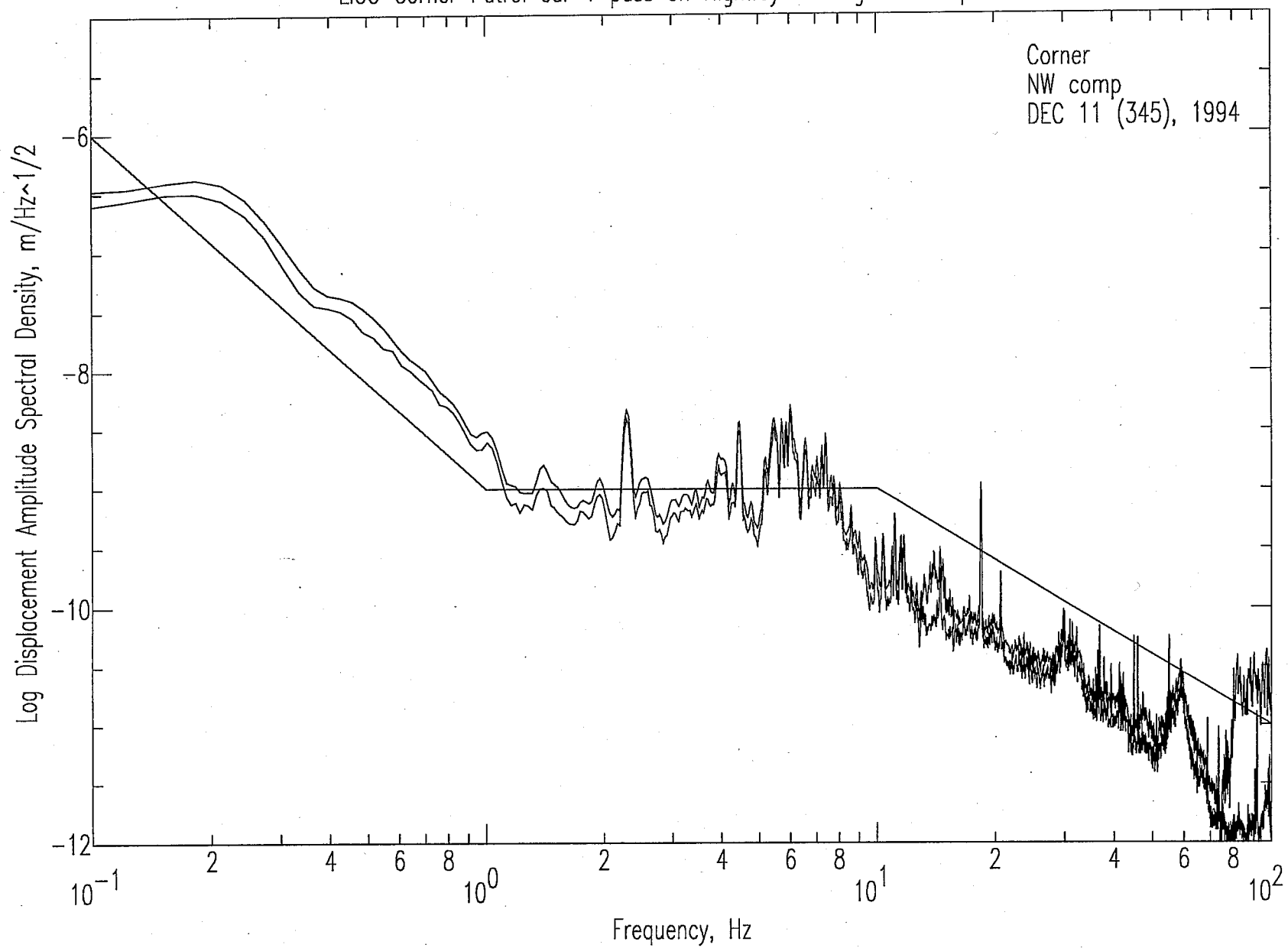
LIGO Corner Patrol car 1 pass on Highway 10 seg0.2.sac Spectra
