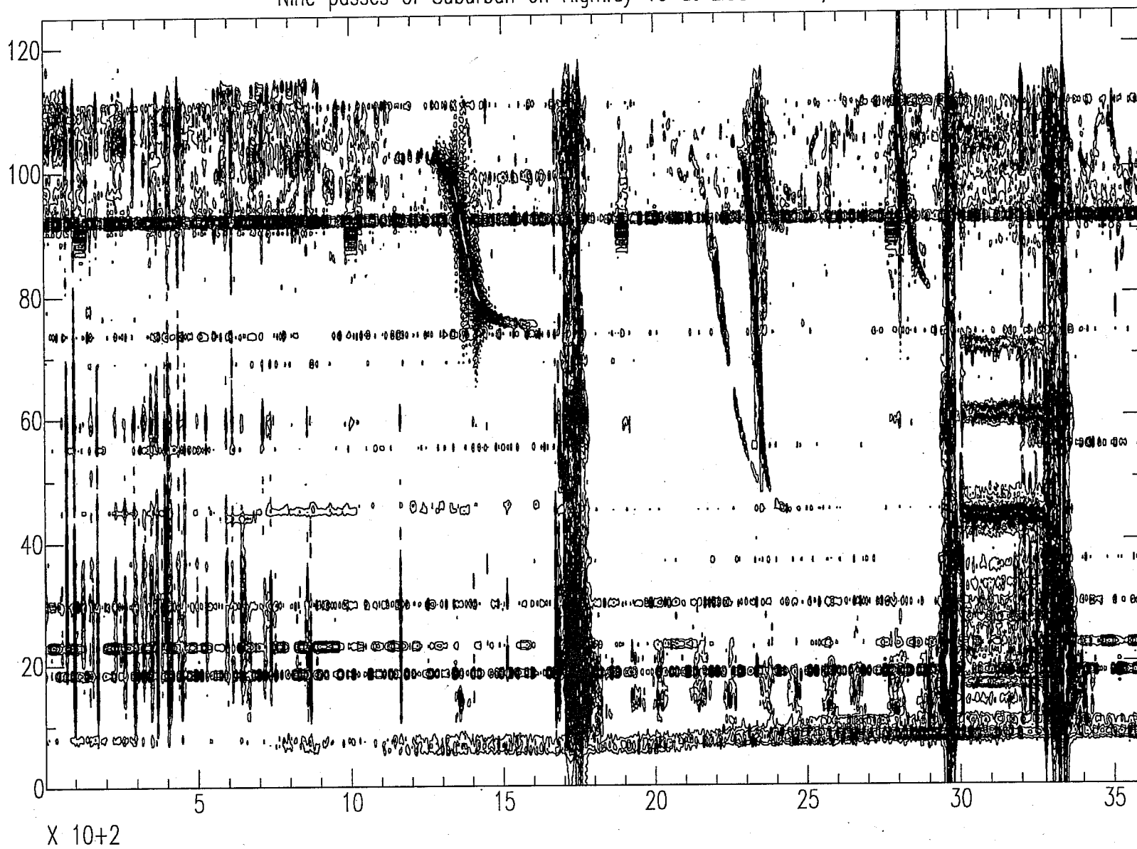
Nine passes of Suburban on Highway 10 at LIGO Corner, Vertical
