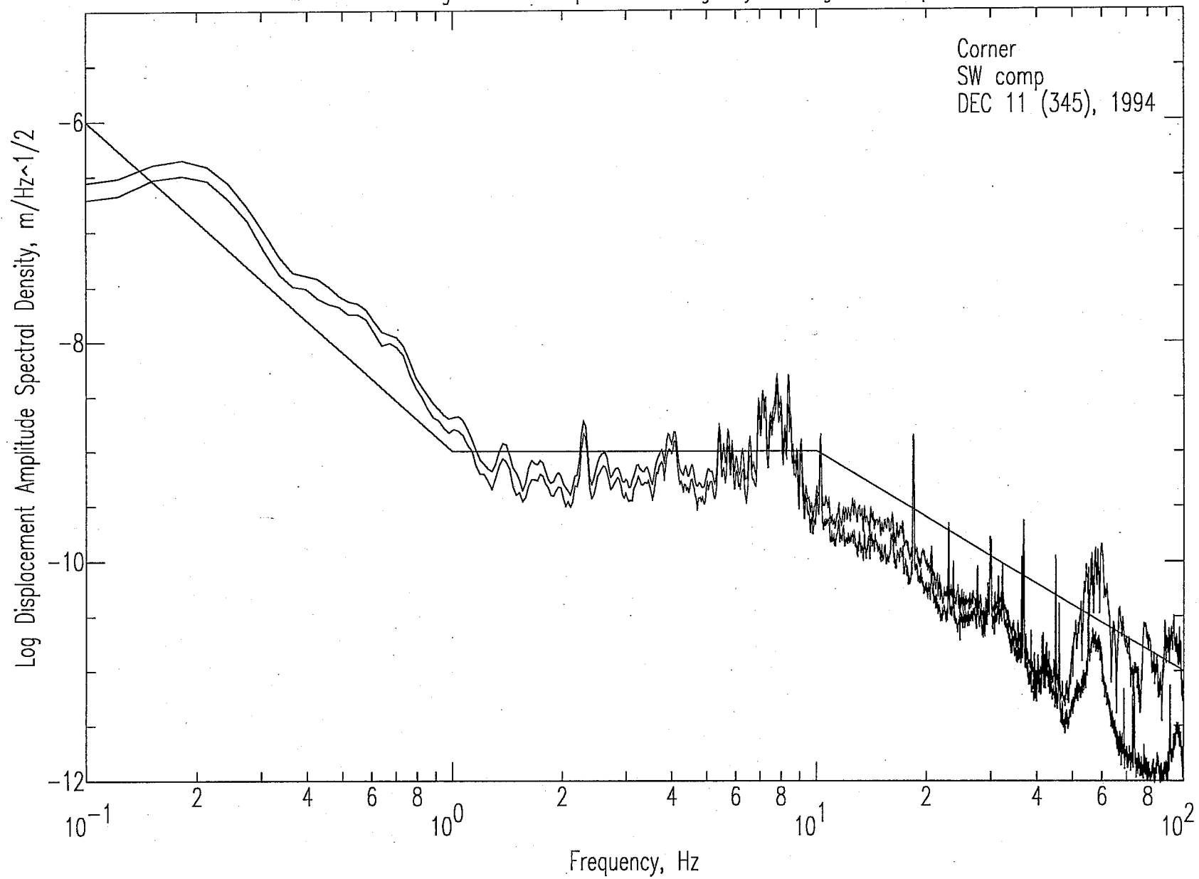
LIGO Corner Single Vehicle 3 passes on Highway 10 seg2.3.sac Spectra
