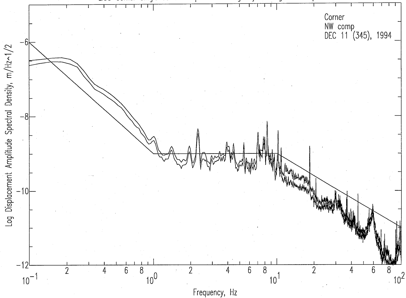
LIGO Corner Single Vehicle 3 passes on Highway 10 seg3.2.sac Spectra
