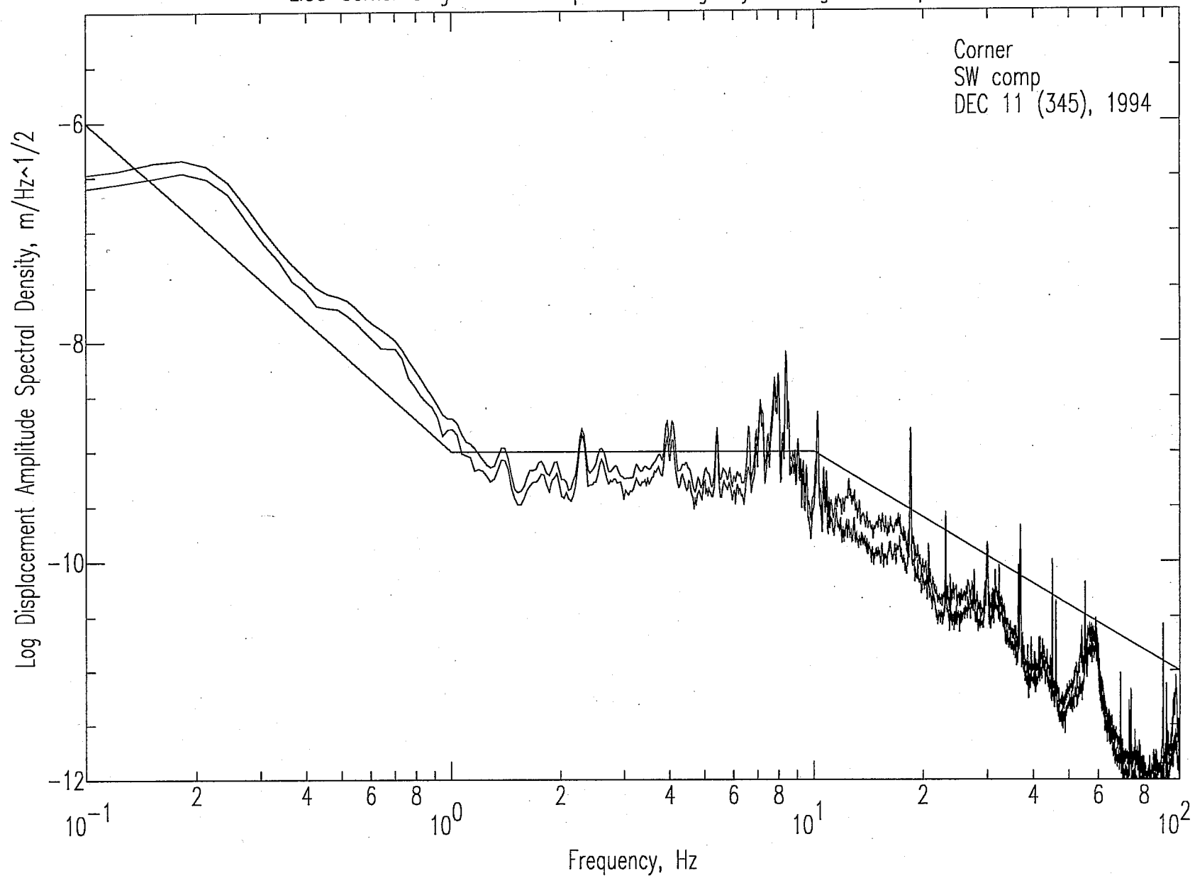
LIGO Corner Single Vehicle 3 passes on Highway 10 seg3.3.sac Spectra
