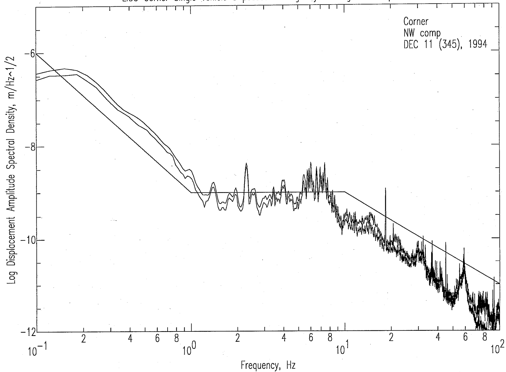
LIGO Corner Single Vehicle 3 passes on Highway 10 seg1.2.sac Spectra
