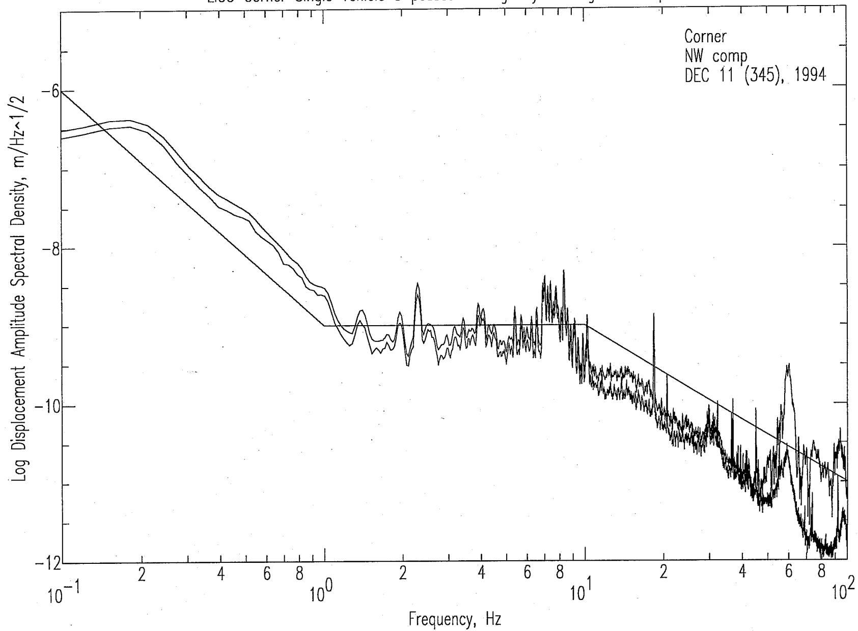
LIGO Corner Single Vehicle 3 passes on Highway 10 seg2.2.sac Spectra
