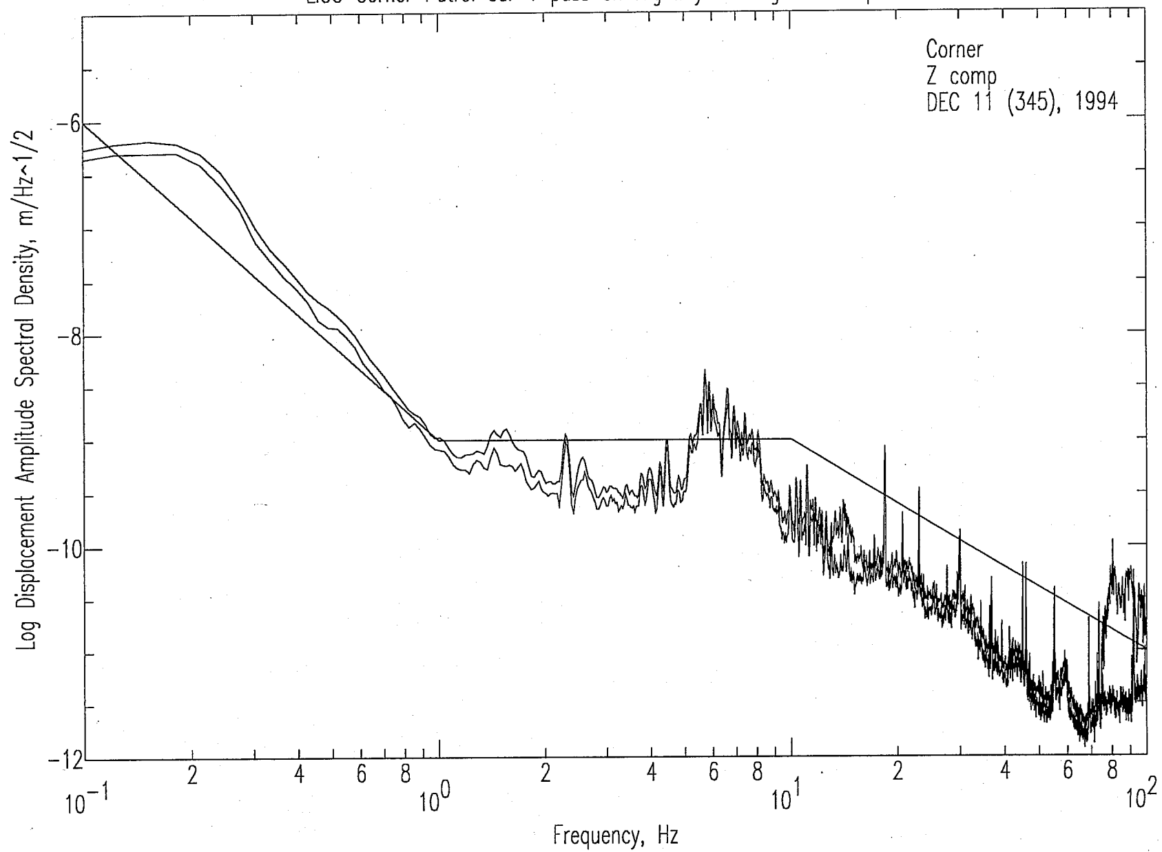
LIGO Corner Patrol car 1 pass on Highway 10 seg0.1.sac Spectra
