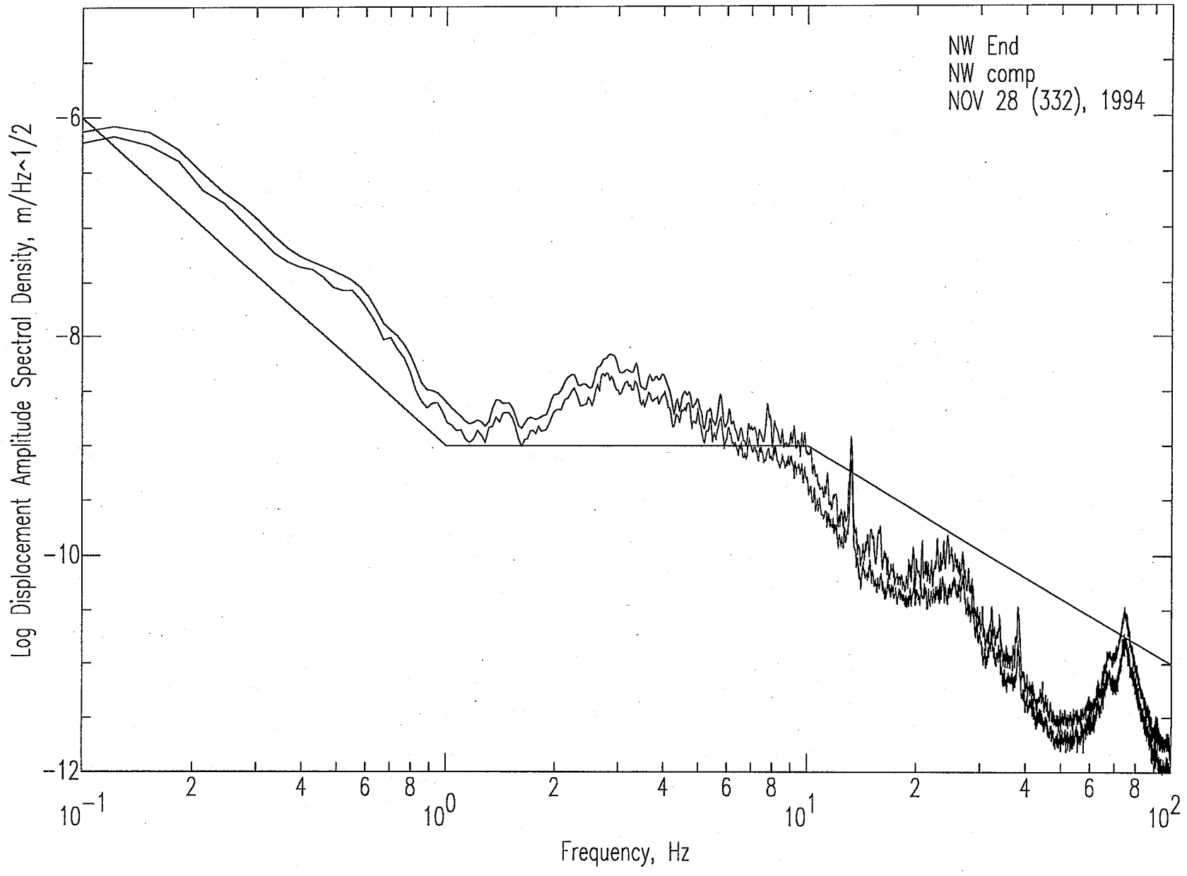
LIGO Construction at 4 km seg2.2.sac Spectra
