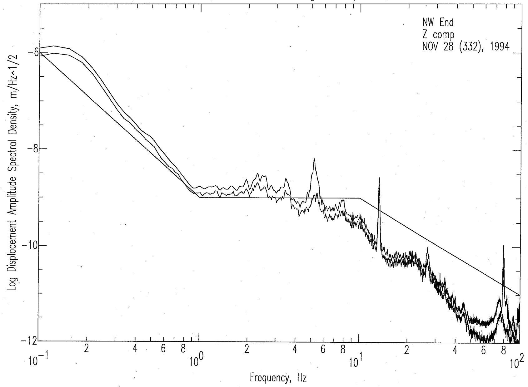
LIGO Construction at 4 km seg4.1.sac Spectra
