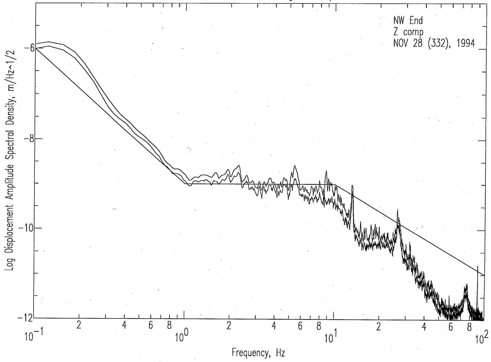
LIGO Construction at 4 km seg3.1.sac Spectra
