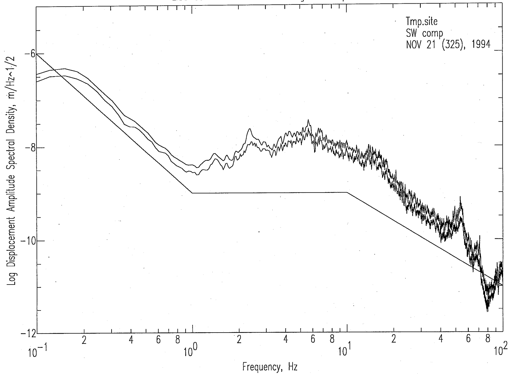
LIGO Construction at 300 m seg4.3.sac Spectra
