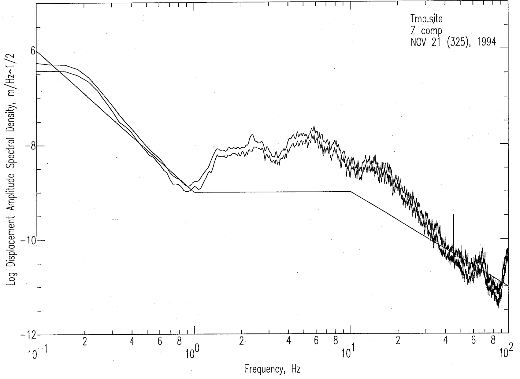
LIGO Construction at 300 m seg4.1.sac Spectra
