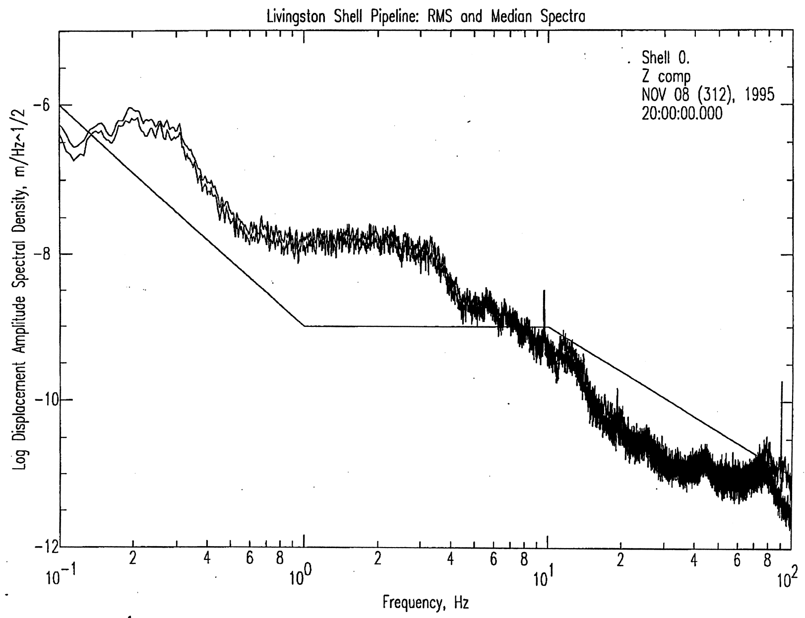
Figure 5. Noise at Shell Pipeline.
