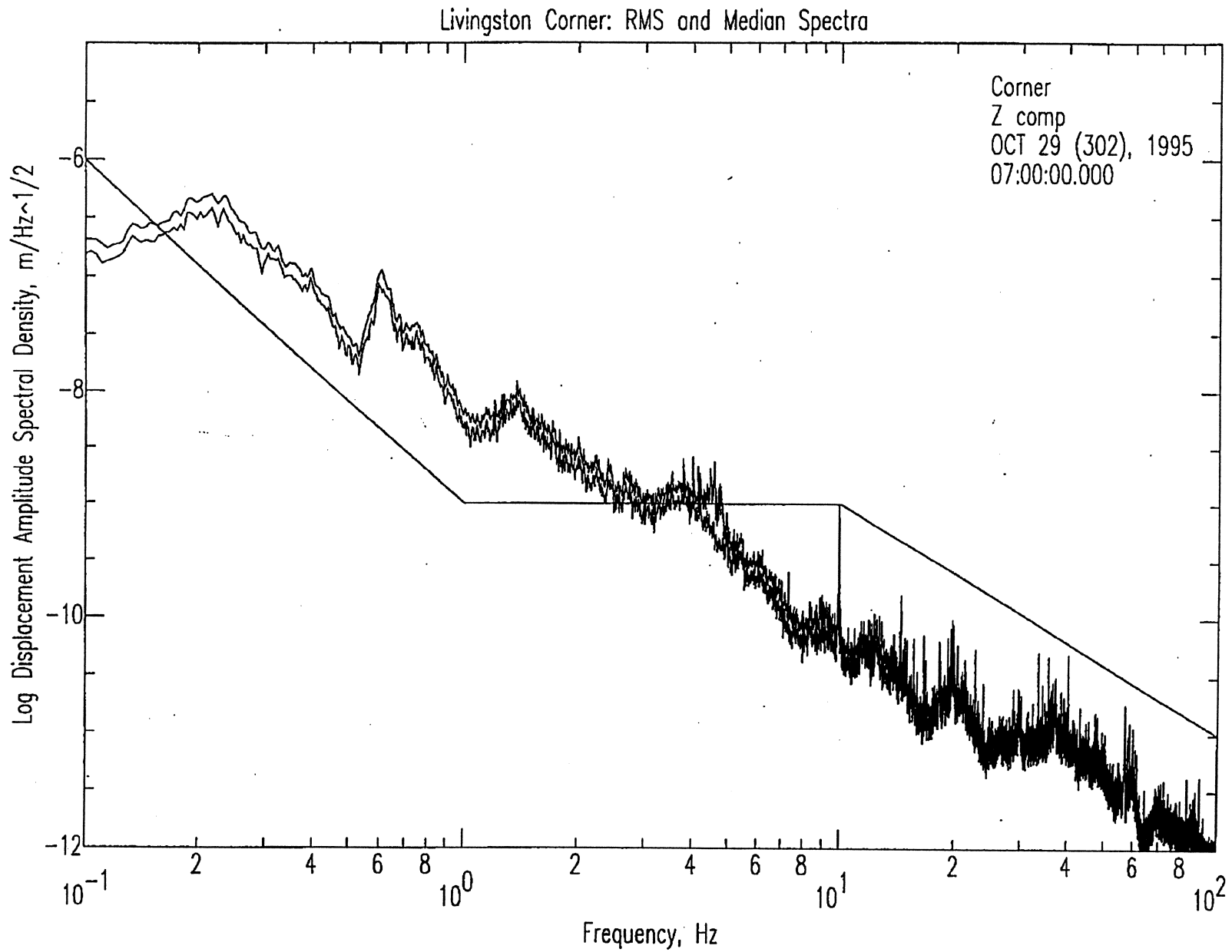
Figure 2. Nighttime seismic noise.
