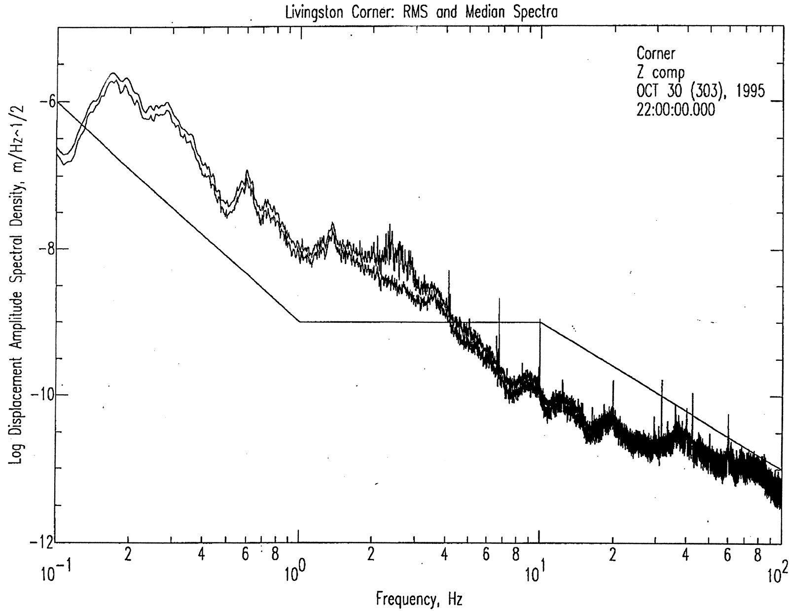
Figure 1. Daytime seismic noise. Figure
