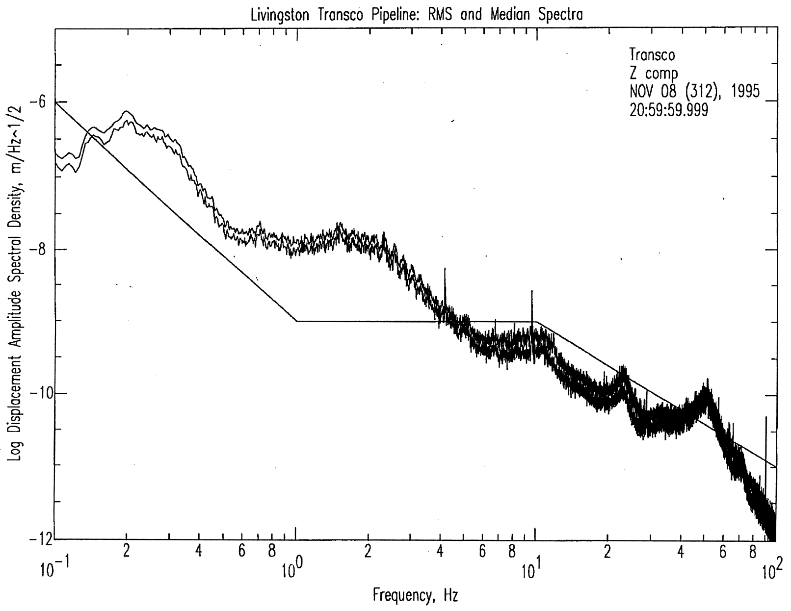
Figure 4. Noise at Transco Pipeline.
