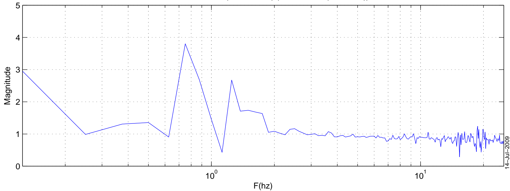
LHO HEPI L4C-V (FFT of CH2)/(FFT of STS2(reference))
