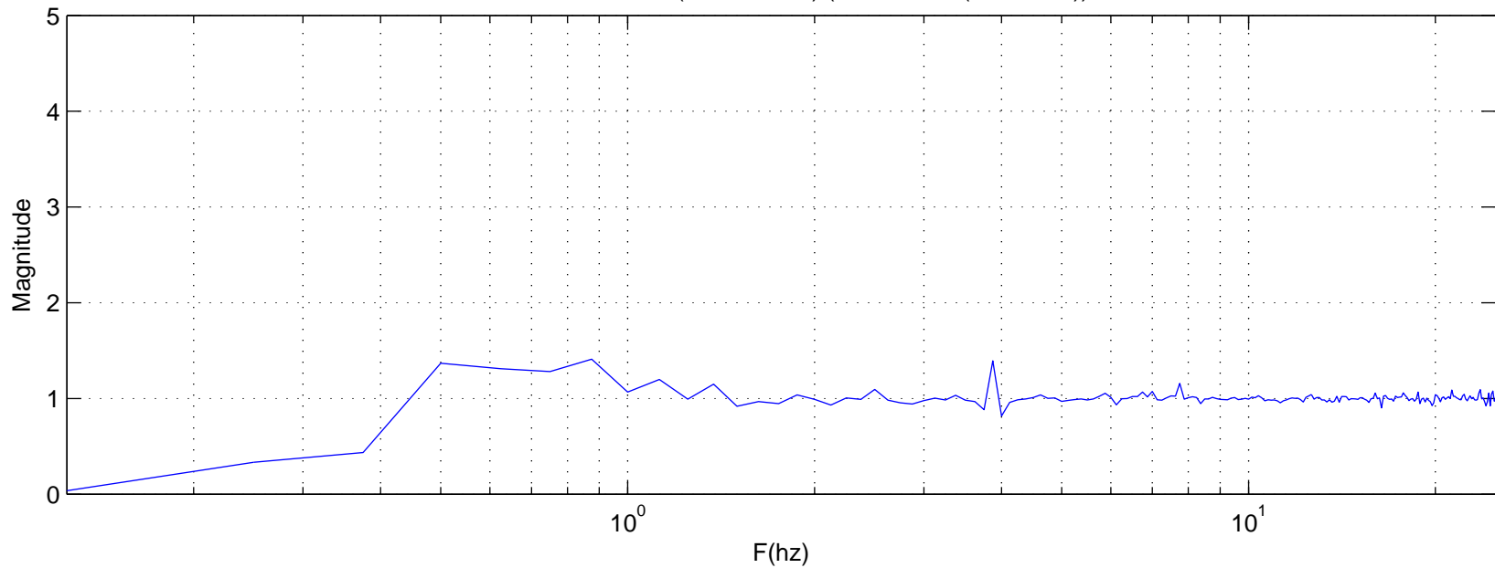
LHO HEPI L4C-V (FFT of CH2)/(FFT of CH1(reference))
