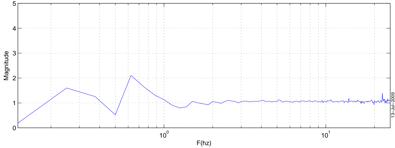
LHO HEPI L4C-V (FFT of CH2)/(FFT of CH1(reference))
