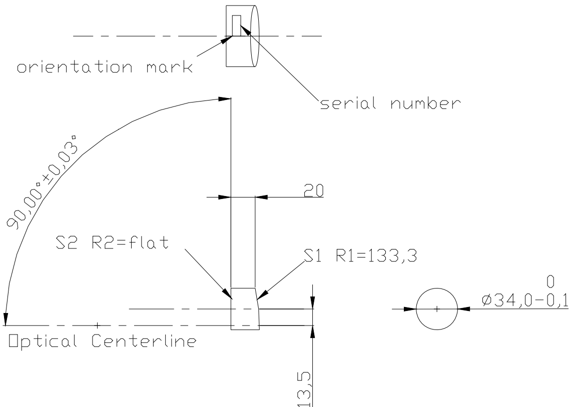
Figure 1: Mirror drawing, parabolic secondary mirror
