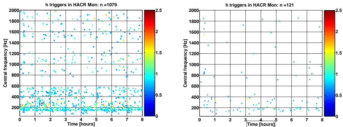
Figure 3. Time-frequency plots of glitch events in the detector output H . The left graph is typical for a time from summer 2006. The right one shows a time from September 2007. Measures that reduced the glitch rate are described in the text.
