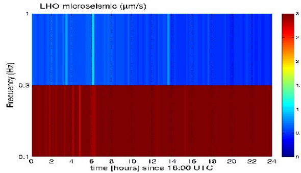
Figure 5. Band-limited seismic noise in the 0.1 - 1 Hz band at Hanford. Such high microseism could cause peaks in the auto-correlogram seen in Fig. 3.
