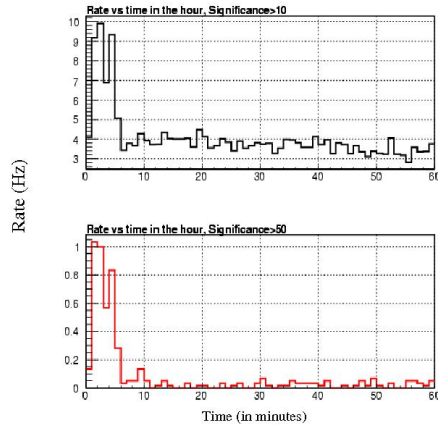
Figure 8. Histogram of the KleinWelle L1 event rate within an hour over a one day period when the detector experienced hourly glitches. The top and bottom panels shows the rate of events with KleinWelle significance greater than 10 and 50 respectively.
