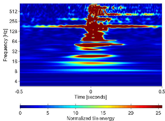
Figure 7. QScan of a glitch in a voltmeter channel, after data whitening with a linear predictive error filter (defined in Ref. [10]).
