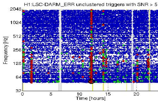
Figure 4. Time-frequency scatter plot of triggers from the QOnline analysis of the 4 km LIGO Hanford detector. The color indicates ranges of SNR with blue indicating SNRs from 5 to 10, green from 10 to 20, and red greater than 20.
