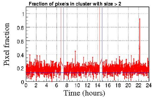
Figure 1. BurstMon [6] pixel fraction as a function of time (with one entry per minute). BurstMon first identifies the most significant 10 percent of time-frequency "pixels" using a wavelet based decomposition of the data. The pixel fraction is defined as the fraction of these significant pixels that can be grouped into clusters of two or more pixels. Ideal noise typically produces isolated pixels, resulting in a typical pixel fraction of 0.13. Pixel fractions much greater than this value indicate a high rate of glitches in the data, which preferentially produce clusters of significant pixels.
