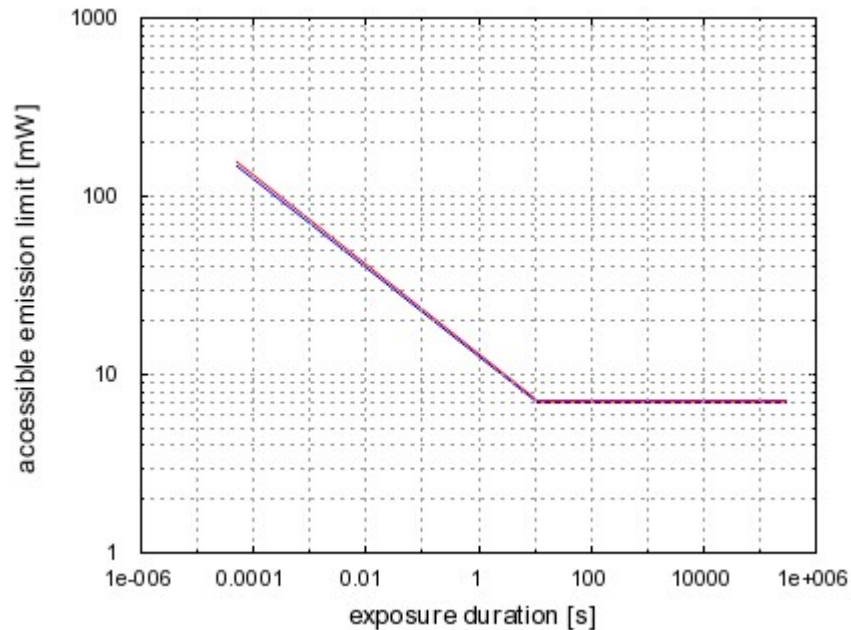
Figure 2. The extended source AEL plotted versus exposure time for the range of angular subtenses considered. The lowest value AEL is (7.0 \pm 0.2) mW.
