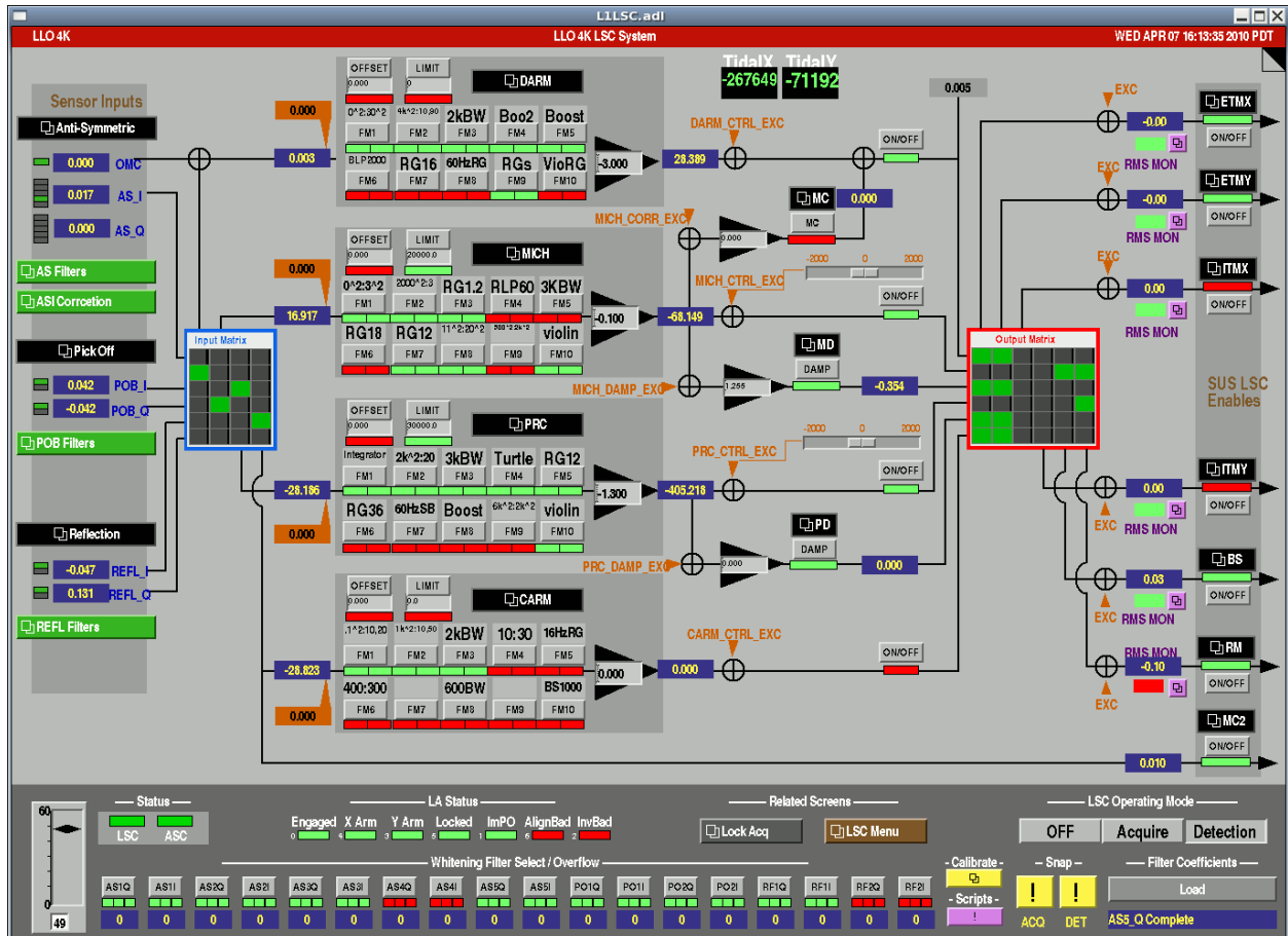
Figure 4.8: The control screen for the Length Sensing and Control subsystem at Livingston. The control screen depicts signal flow in a generally left-to-right manner. Photodiodes at the anti-symmetric (AS), pick-off (PO), and reflected (REFL) ports are indicated on the extreme left. These signals are combined via an input matrix to form the DARM, MICH, PRC, and CARM degrees of freedom. These signals are processed through an array of filter banks defining the control filters. Finally, the signals pass through an output matrix and are then directed to the individual optics.
