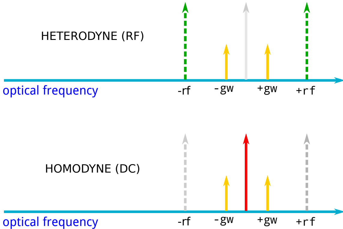
Figure 3.3: Depiction of the fields in DC and RF readouts. (a) In RF readout, the laser carrier is suppressed by operating the Michelson on a dark fringe for the carrier. Differential phase modulation in the arms becomes amplitude modulation of the (suppressed) carrier, depicted as the audio-frequency sidebands at \pm f_{gw} . The photodiode sees a beat between the GW signal and the RF sidebands. In homodyne readout, a carrier-frequency local oscillator is introduced—in DC readout this is done by introducing a microscopic asymmetry between the two arms. The RF sidebands are no longer needed and are removed by the output mode cleaner. The GW-induced sidebands appear as amplitude modulation on the carrier, which is sensed directly by the photodiodes.
