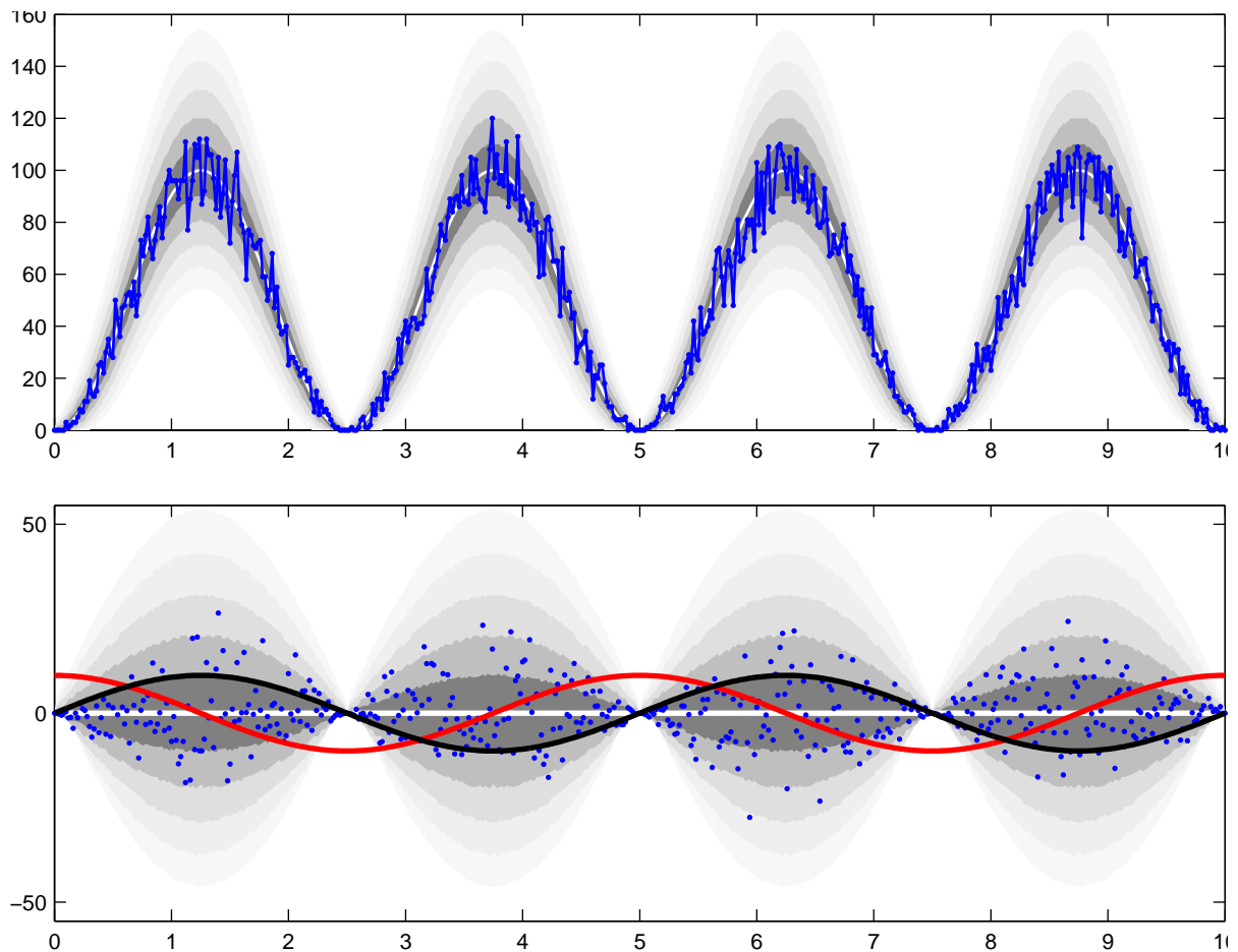
Figure 2.7: (a) Model of shot noise in the presence of sinusoidal power modulation, as occurs in optical heterodyne detection. The photodiode sees a power modulation at 2f_{mod} (white) due to the beat between the upper and lower modulation sidebands at f_{carrier} \pm f_{mod} . The gray levels represent the 1\sigma , 2\sigma , \dots , 5\sigma ranges for a Poisson distribution. The blue dots are a sample realization of this noise. (b) Subtracting the mean from (a) leaves only the noise; its bursty nature is obvious. Shown in black and red are the I and Q demodulation waveforms, respectively. It is clear that the in-phase demodulation (I) samples regions of the time series with higher variance than the quadrature phase (Q). This leads to a higher variance (shot noise level) in the I signal and a lower one in the Q signal relative to what one would expect from a naïve assumption based on the average power considered over a whole period of the waveform.
