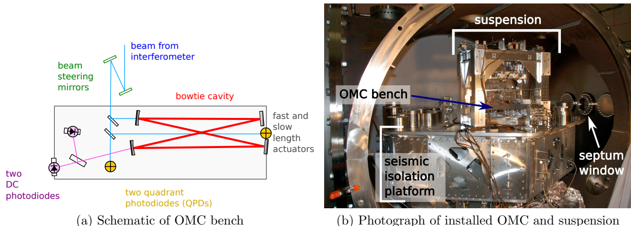
Figure 4.2: (a) Diagram illustrating the design of the monolithic OMC bench; (b) Photograph of the installed output mode cleaner, suspension, and seismic isolation platform. The OMC is located in a dedicated vacuum chamber, separated from the main vacuum enclosure by a septum window, allowing rapid venting cycles during commissioning.
