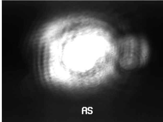
Figure 4.1: Image of the beam spot at the L1 output port taken using a CCD camera. This image is saturated in the central portion but emphasizes the spurious higher order modes surrounding the fundamental Gaussian, including contributions from both the carrier and the 25 MHz sidebands.
