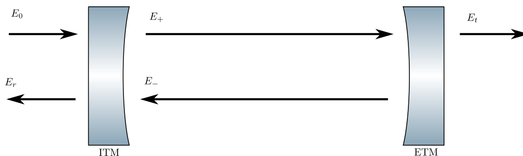
Figure C.1: Fabry-Perot cavity. When used as an arm cavity, the two mirrors are known as the input (ITM) and end (ETM) test masses. Here E_0 indicates the amplitude of the incident electric field, E_r the reflected field, E_+ the forward-going intra-cavity field, etc.
