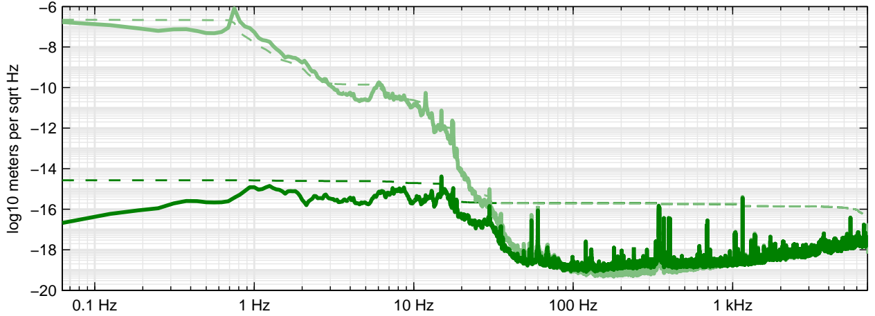
Figure 3.5: DARM motion. The lower trace shows the residual motion of DARM after stabilization by the DARM control loop. The upper trace shows the ‘calibrated’ DARM, in which the effect of the control loop has been removed by multiplying by (1 + G) , where G is the open loop gain; this can be interpreted as ‘the motion that would be there if there were no control loop.’ The control loop reduces the RMS DARM motion by ten orders of magnitude in order to hold the interferometer within the linear regime around the operating point. The DARM offset used to implement DC readout must be significantly larger than the RMS residual motion ( \sim 10^{-14} m) to avoid nonlinear effects.
