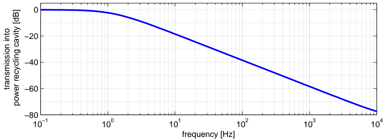
Figure 2.4: Transfer function from laser intensity fluctuations incident on the interferometer to laser intensity fluctuations inside the power recycling cavity. Fluctuations around the laser carrier above the coupled-cavity pole are attenuated.
