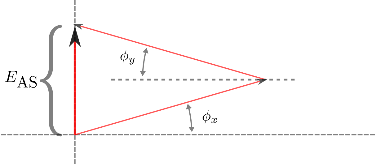
Figure 2.2: Phasor diagram of the fields at the output port due to the two arms of the Michelson. Differential motion of the mirrors at the ends of the arms causes equal but opposite rotation of the two phasors, which modulates the amplitude of the resultant electric field at the output port ( E_{AS} ).
