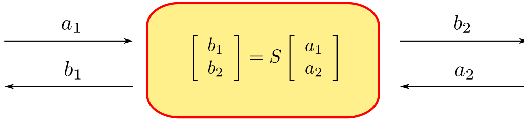
Figure E.1: The scattering matrix S gives the amplitudes of the outgoing fields b_1 and b_2 in terms of the in-going fields a_1 and a_2 .
