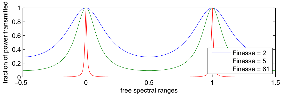
Figure C.3: Power transmission coefficients for three critically-coupled cavities.
