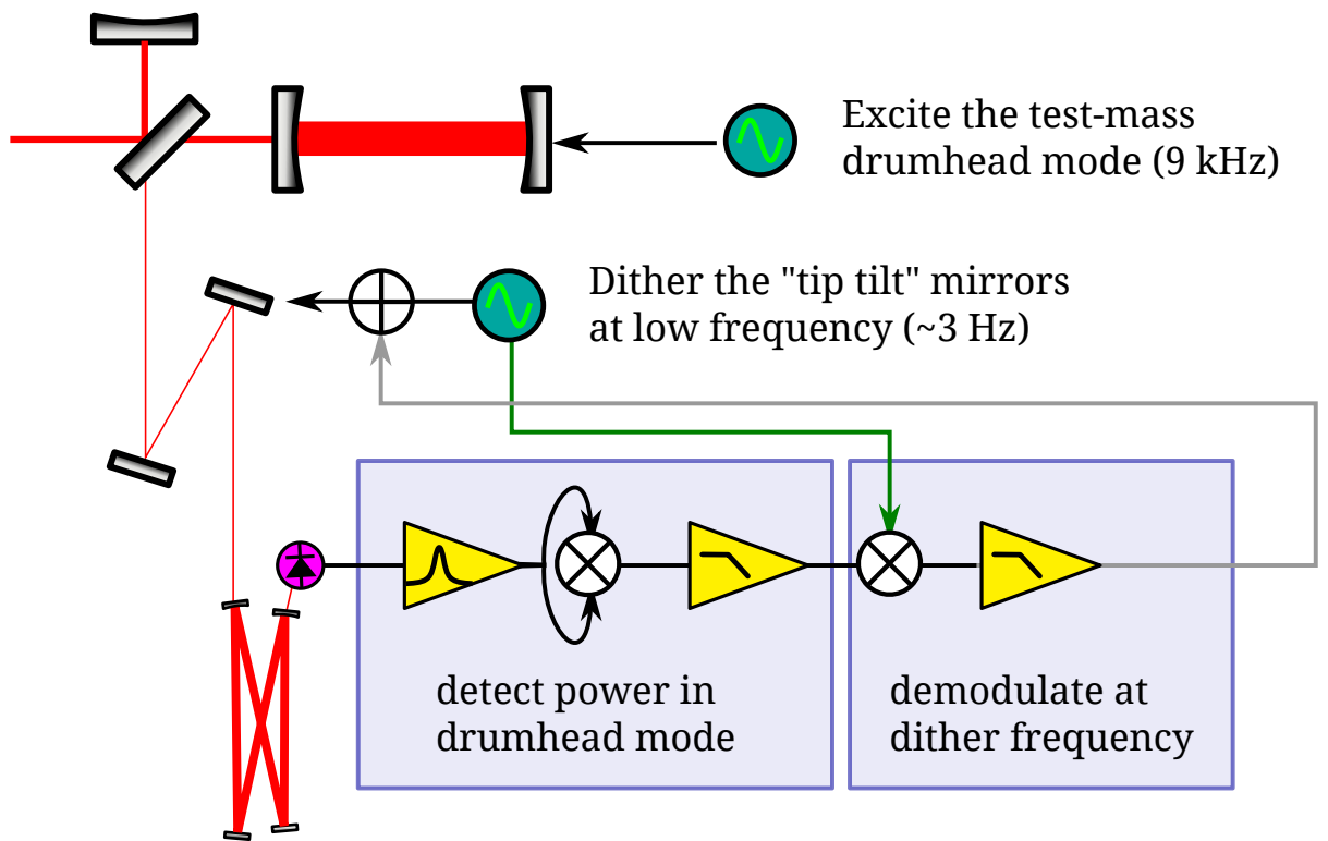
Figure 4.6: The 'Drumhead dither' OMC alignment system.
