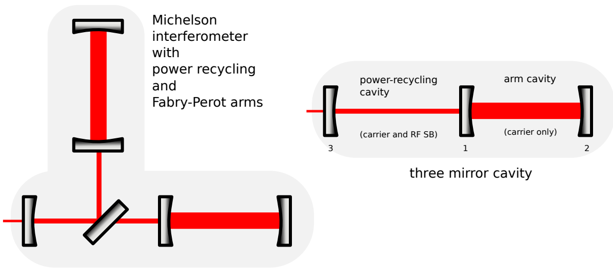
Figure 2.3: It is sometimes convenient to condense the two arms of the Power-Recycled Fabry-Perot Michelson interferometer into a single ‘virtual arm’ for the purpose of analysis.
