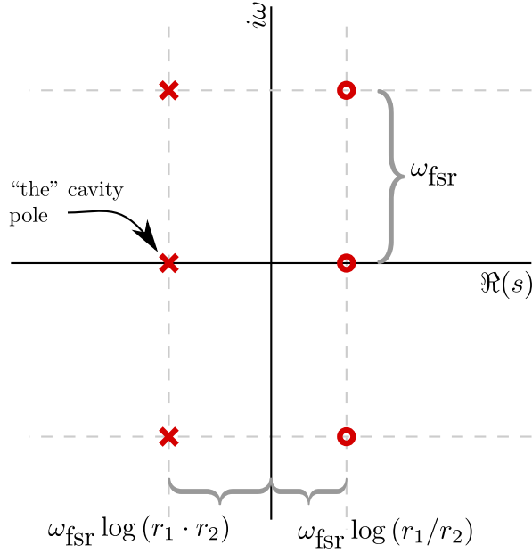
Figure C.2: Pole-zero map of the cavity amplitude reflectivity. Poles are designated with \times and zeros with \circ ; r_1 is the amplitude reflectivity of the input coupler, and r_2 is the amplitude reflectivity of the output coupler. Losses can be lumped into r_2 . Notice that the free spectral range (angular frequency \omega_{\text{fsr}} ) sets the scale of the entire diagram, and the function is periodic in i\omega : there is an infinite line of poles and an infinite line of zeros. Two limiting cases are worth considering: (1) A critically-coupled cavity has r_1 = r_2 , which brings the line of zeros onto the imaginary axis. On resonance, i\omega travels through these zeros and the cavity reflectivity vanishes. This models the desired behavior of mode cleaner cavities. (2) A maximally over-coupled cavity has r_2 = 1 , in which case the line of poles and line of zeros are equally spaced from the imaginary axis. This models the LIGO arm cavities. The cavity’s amplitude transmission has the same poles as the reflectivity but no zeros.
