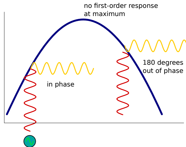
Figure 4.4: Cartoon view of dither locking. The dither locking technique allows a system to be locked to a quadratic operating point. For example, dither locking is used to control the OMC cavity length, where, near resonance, transmission is a quadratic function of cavity displacements. A sinusoidal modulation is injected into the parameter we wish to tune (i.e. cavity length), and the output (i.e. transmitted light intensity) is demodulated at the same frequency, producing an error signal. The figure shows the phase-flip that occurs as the system moves through the quadratic point. At the quadratic point, the error signal is zero, while on either side it attains nonzero values with opposite signs.
