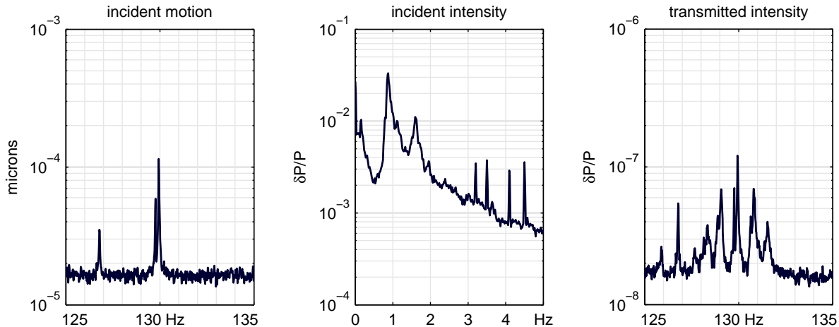
Figure 5.8: Example of linear and bilinear beam jitter coupling in the L1 OMC. Left: the light incident on the OMC shows motion at \sim 130 Hz (arbitrary units). Center: the incident light contains intensity modulations at \sim 0.87 and \sim 1.6 Hz (units: \log_{10}(\delta P/P) ). Right: the light transmitted through the OMC contains intensity modulations at 130 Hz, 130 \pm 0.87 Hz, and 130 \pm 1.6 Hz (units: \log_{10}(\delta P/P) ). (The sources of the incident beam motion and intensity fluctuations have not been identified.)
