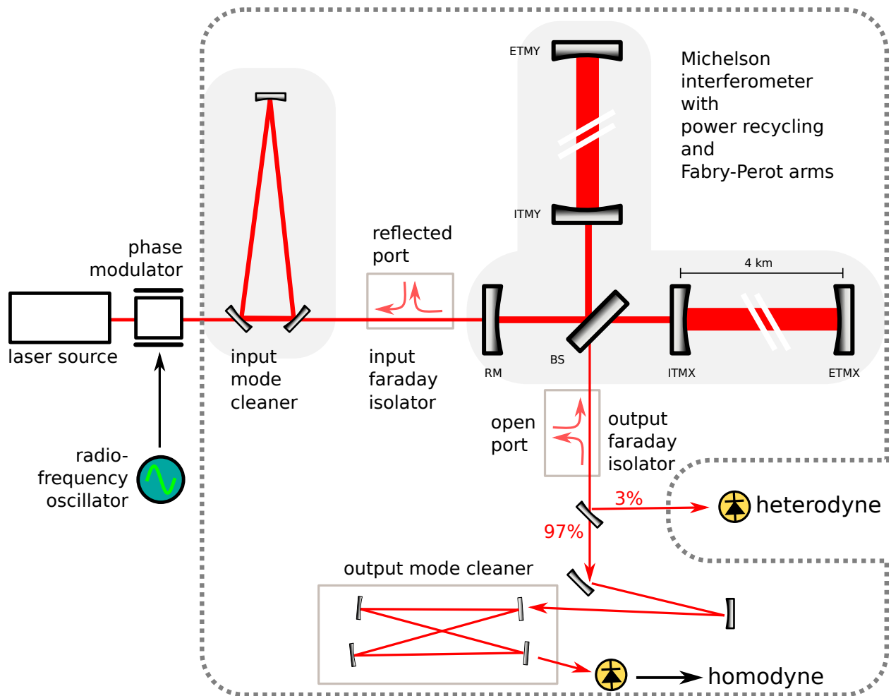
Figure 3.4: Enhanced LIGO interferometer layout (not to scale). The dotted line represents the vacuum enclosure.
