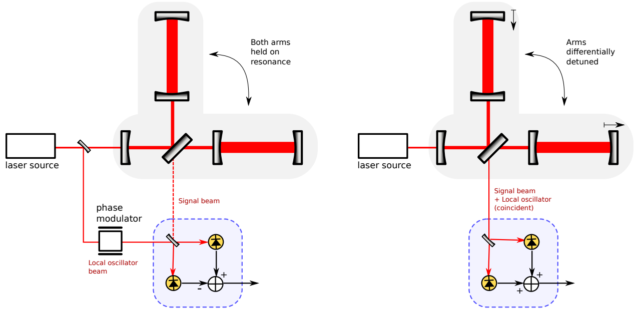
Figure 3.1: Left: a traditional ‘balanced photodiode’ homodyne detection arrangement. Right: DC readout with two photodiodes.
