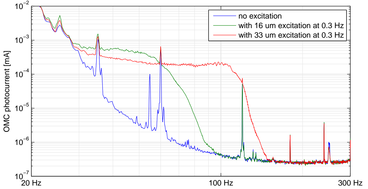
Figure 4.7: Measurement of effective OMC backscattering reflectivity. With the interferometer operating in low-noise mode, we excited (modulated) the position of the OMC in the direction of the incident beam, thus modulating the path length between the interferometer and the OMC. This produces the characteristic ‘scattering shelf’ spectrum in the power at the OMC photodiodes. Integrating the area under the shelf and dividing by the DC power gives the effective backscattering reflectivity. (The photocurrent has been corrected for the suppression of the DARM control loop.)
