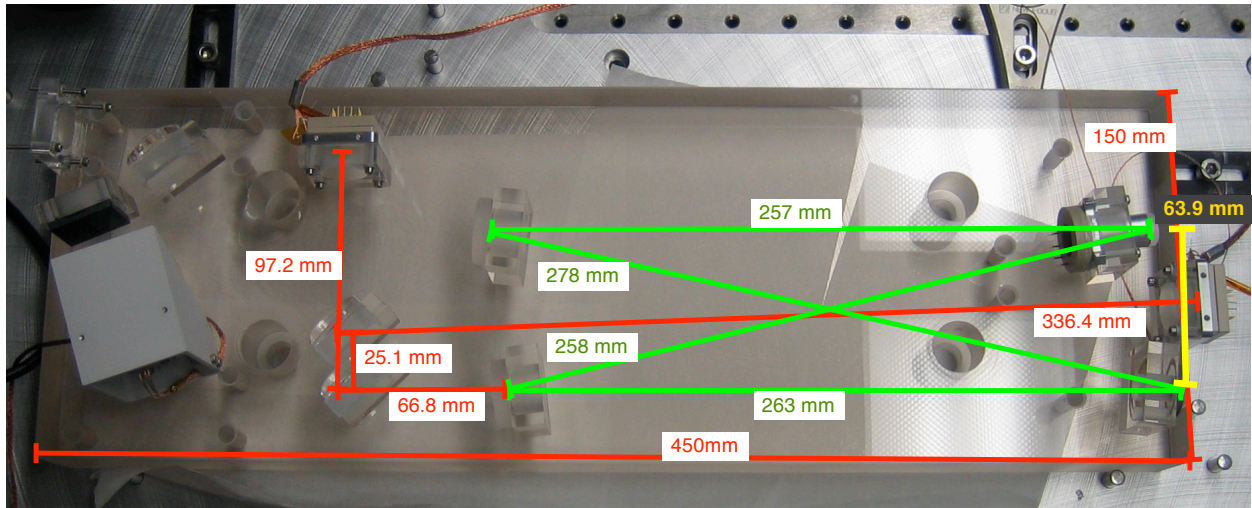
Figure 4.3: Photograph of the Output Mode Cleaner used at Livingston ( ex situ ). Only one of the two DC photodiodes is installed in this photo. Photometry by Sam Waldman; this diagram has document number D0901817.
