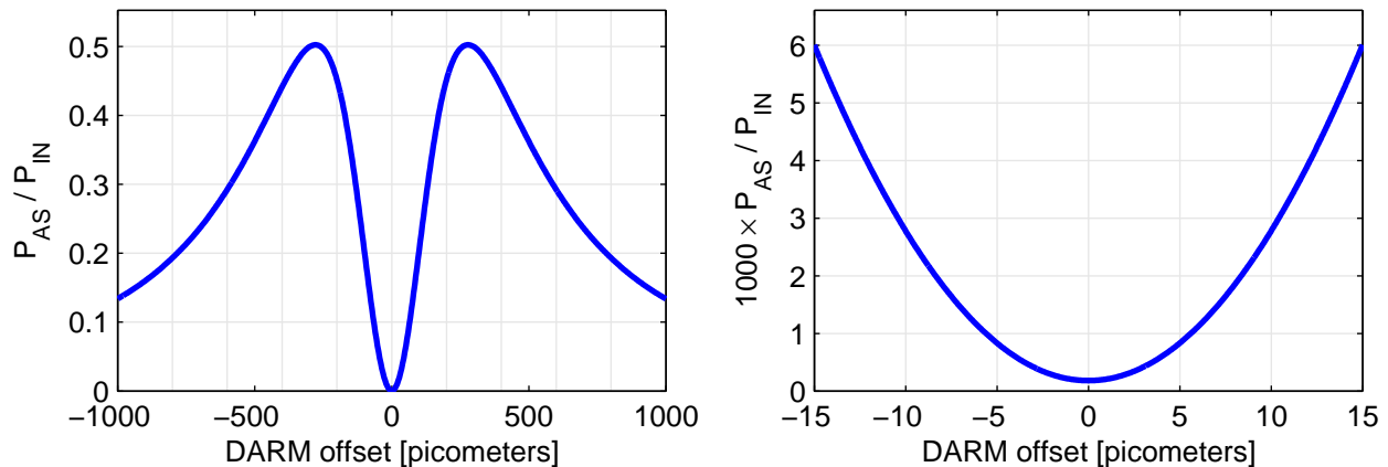
Figure 3.2: Power at the output port ( P_{AS} ) relative to the interferometer input power ( P_{IN} ), as a function of the DARM offset, in picometers ( 1 \text{ pm} = 10^{-12} \text{ m} ). Left: The DARM fringe differs from the P_{BS} \sin^2 kx of a simple Michelson since P_{BS} itself depends on the DARM offset. For comparison recall that the full fringe width (from one resonance to the next) is \lambda \approx 10^{-6} \text{ m} . Right: Detail. For small offsets, the fringe appears quadratic. DC readout operates with an intentional static DARM offset in order to create a linear relationship between DARM perturbations and P_{AS} . The small but nonzero minimum power at zero offset is the contrast defect.
