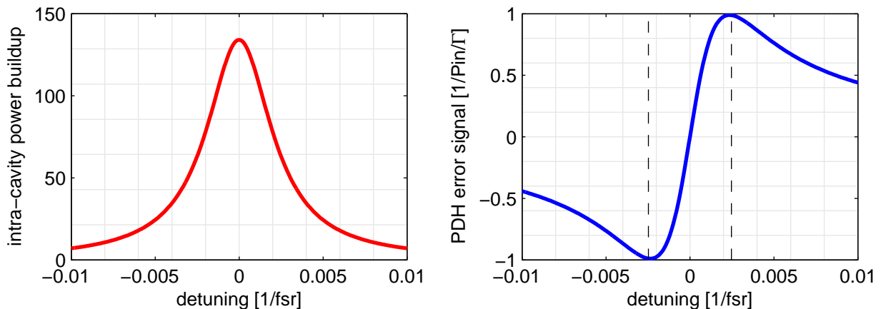
Figure 2.6: (a) Power buildup inside a resonant cavity relative to the incident power, as a function of cavity detuning (deviation from resonance). (b) The Pound-Drever-Hall error signal as a function of detuning (in watts relative to the incident power and the modulation depth). The dashed lines indicate the region in which PDH provides a usable error signal with which to lock the cavity. The cavity modeled here has parameters similar to the initial LIGO arm cavities.
