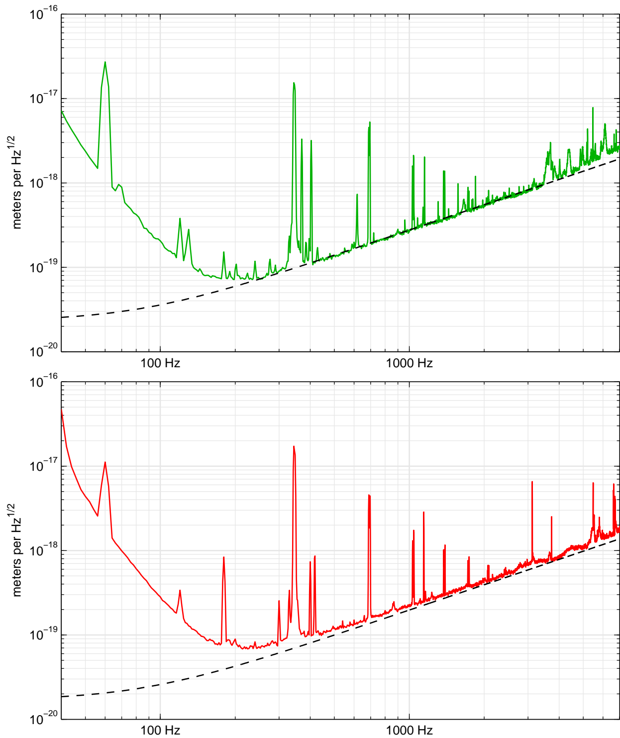
Figure 5.1: Shot noise limited sensitivity of the Livingston and Hanford detectors. The uncertainty in the measured displacement spectra is \sim 10\% , and in the modeled curves is \sim 20\% .
