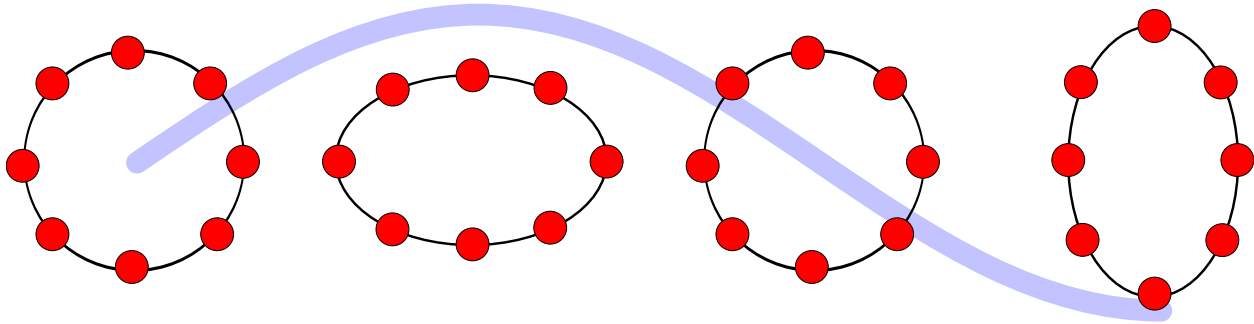
Figure 1.1: Effect of a gravitational wave (traveling into or out of the page) on a ring of non-interacting inertial test particles, with the gravitational wave waveform superimposed.
