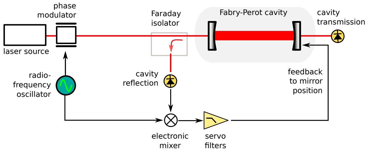
Figure 2.5: In the basic Pound-Drever-Hall setup, a phase modulator is used to produce RF sidebands well outside of the cavity bandwidth. The light reflected from the cavity is incident on a photodiode, the signal from which is demodulated to produce an error signal indicating the mismatch between cavity length and laser carrier frequency. Through feedback, the cavity can be ‘locked’ to the resonance. The technique can be generalized to sense and control much more complex interferometers.
