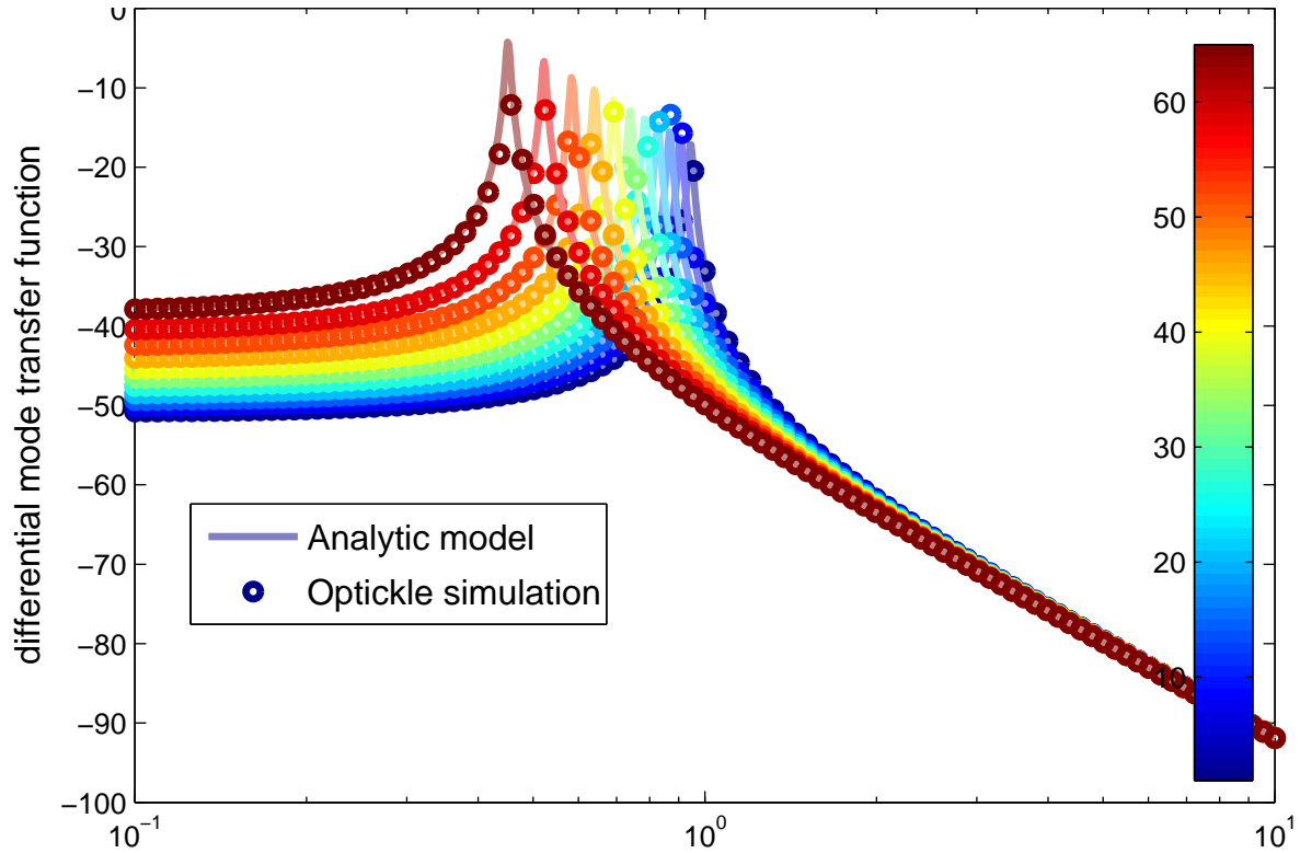
Figure D.1: The optical spring effect: As a cavity is detuned from resonance, the resonance of the differential mode decreases. This figure compares the results of a numerical (Optickle) model with analytic results. The units of the y-axis are 20 \log_{10}(\text{displacement/force}) ; the x-axis is Hz; color indicates cavity detuning in picometers.
