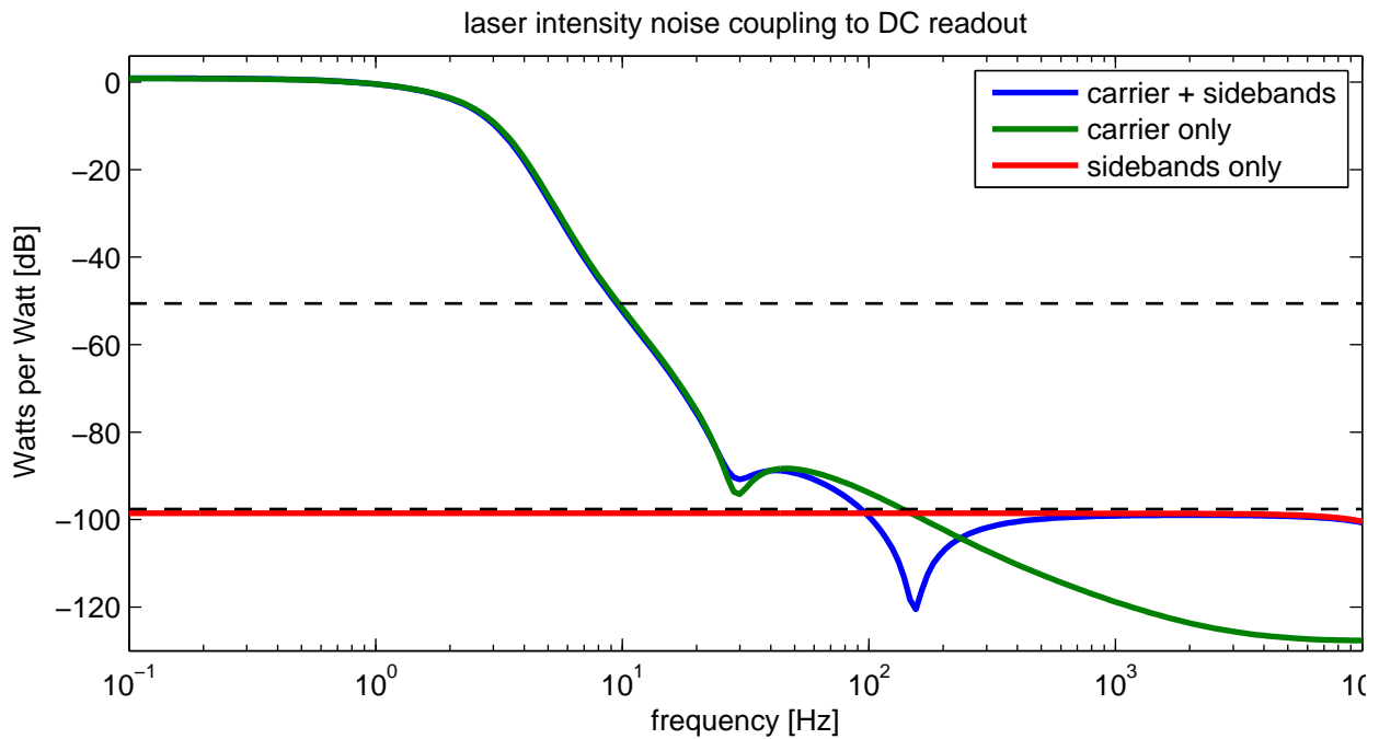
Figure 5.3: Direct contributions of amplitude modulation of the laser carrier and RF sidebands to DC readout, in the absence of radiation pressure. The carrier contribution is shaped by the coupled cavity pole. The RF contribution is due to residual off-resonance transmission through the OMC. Interference between the two coupling mechanisms creates a dip in the total coupling at the crossover frequency.
