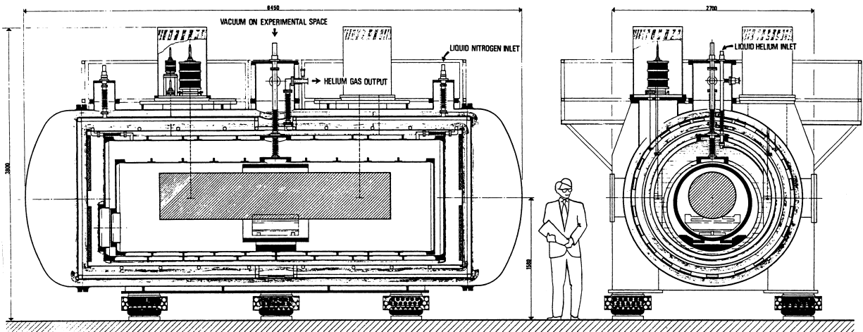
Figure 1.2: Depiction of the cryostat of the EXPLORER bar detector, which has operated at CERN since 1990. EXPLORER was oriented in parallel to the ALLEGRO detector at LSU[9] to enable searches for coincident detections. Illustration adapted from [10].
