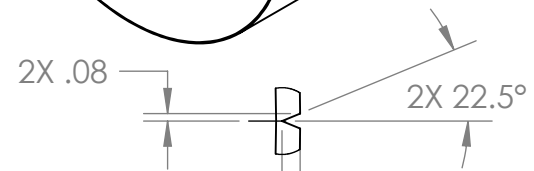
DETAIL A SCALE 1 : 2 WELD PREP DETAIL
