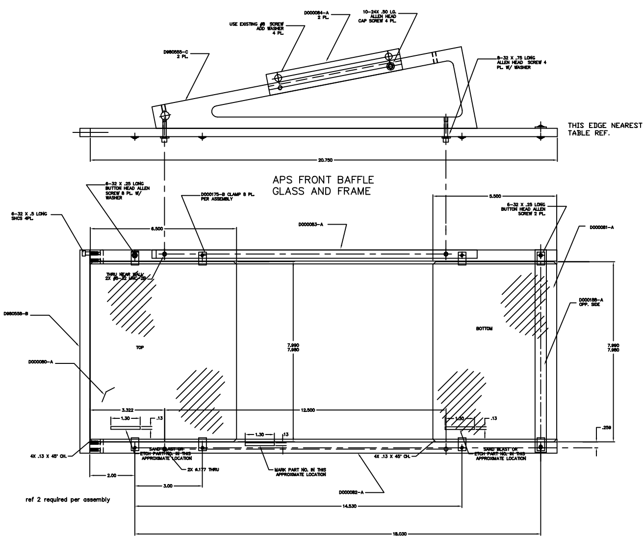
APS 2K BAFFLE SEE D000246 FOR 4K BAFFLE
