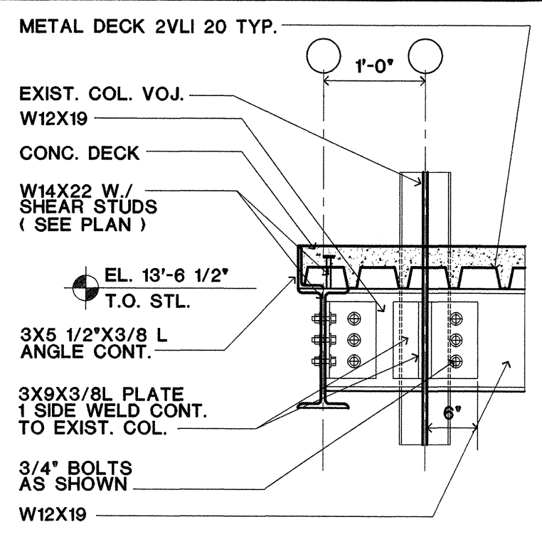
1 DETAIL 3/4" = 1' - 0" TYPICAL
