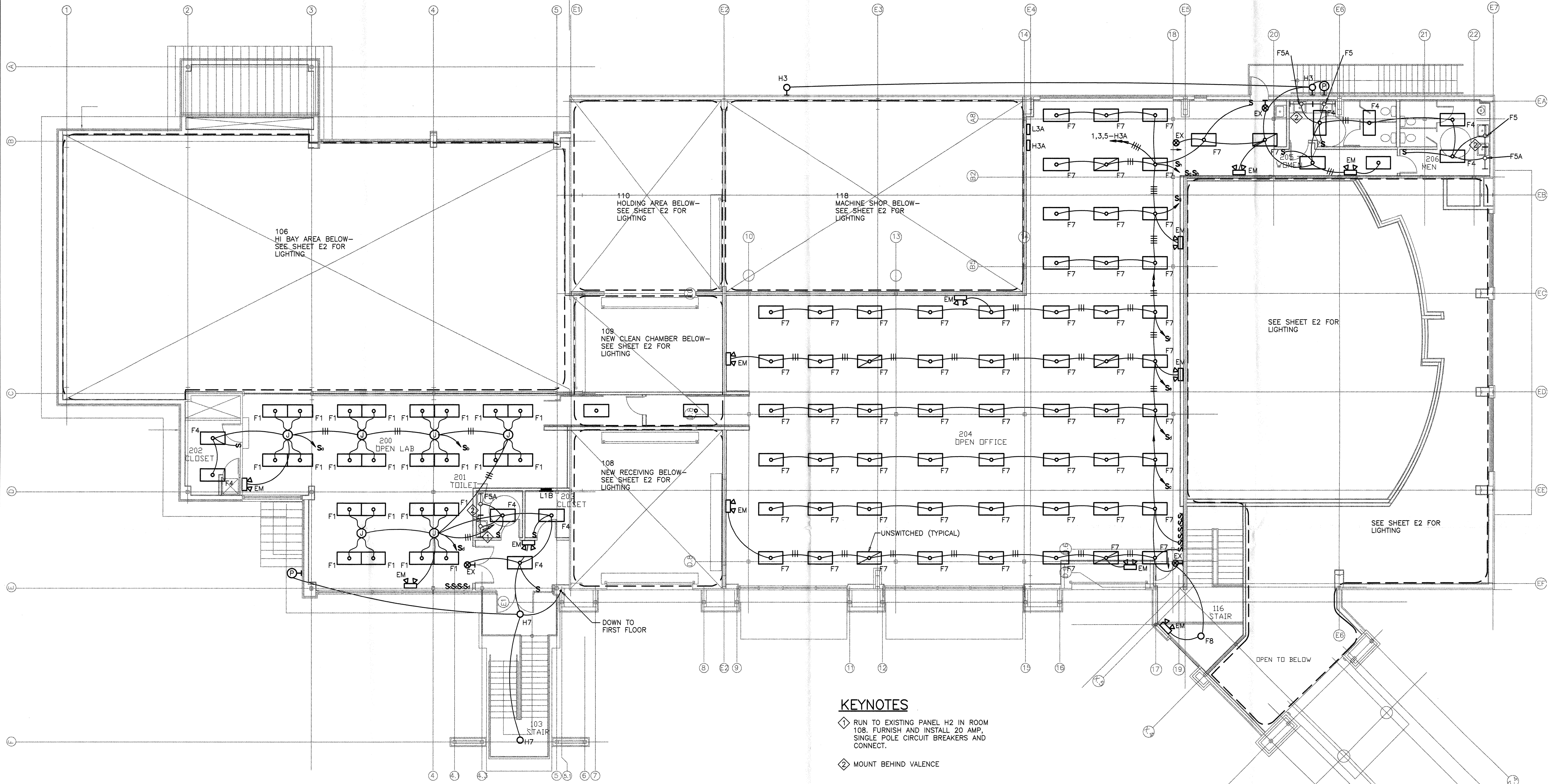
SECOND FLOOR PLAN - LIGHTING 1/8" = 1'-0"
