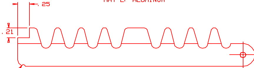
BOTTOM BAR 1 REQ'D PER ASSEMBLY MAT'L: ALUMINUM
