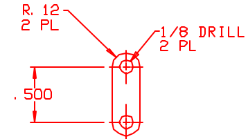
LINK 2 REQ'D PER ASSEMBLY MAT'L: STAINLESS STEEL
