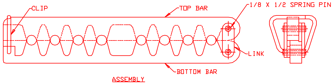
ASSEMBLY
