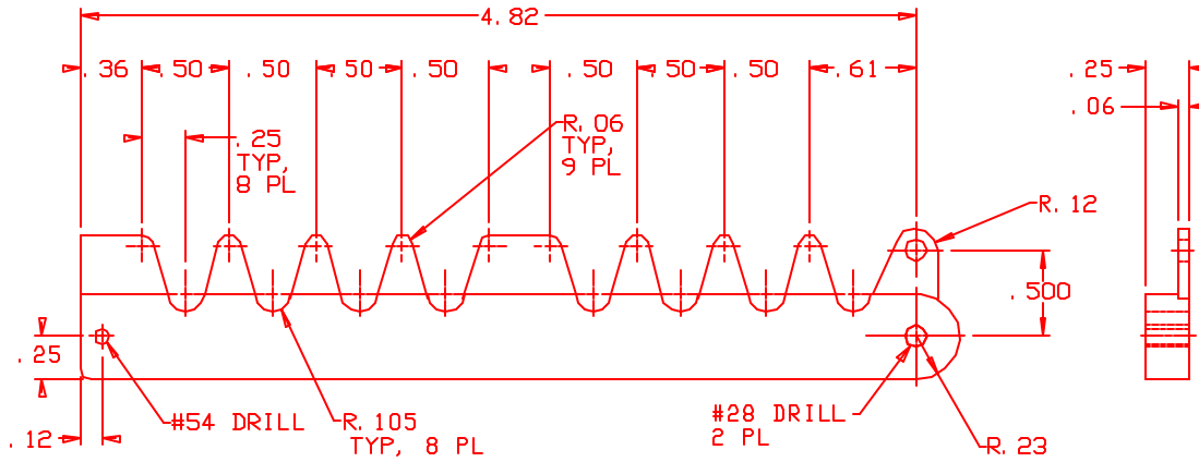
BOTTOM BAR 1 REQ'D PER ASSEMBLY MAT'L: ALUMINUM
