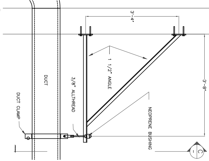
1 DUCT SUPPORT DETAIL SCALE: 1" = 1'-0"
