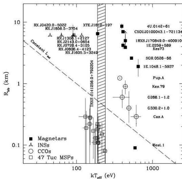
Figure 6.2: Figure reproduced with permission from [115]. Plot of effective temperature kT_{\text{eff}} vs blackbody radius R_{bb} . Best fits for Calvera lie in the hashed region. All four possibilities are plotted on the same plot, so comparisons can be made with Calvera.
