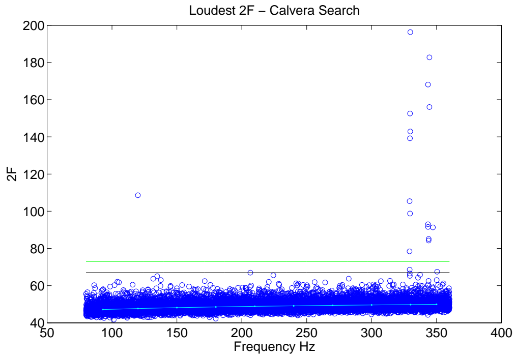
Figure 7.8: The raw results of the search. The maximum 2\mathcal{F} is shown for each frequency band. The black line is the expected loudest 2\mathcal{F} for the whole search. The green line is the 1% false alarm rate threshold. The cyan line is the expected loudest 2\mathcal{F} for each band.
