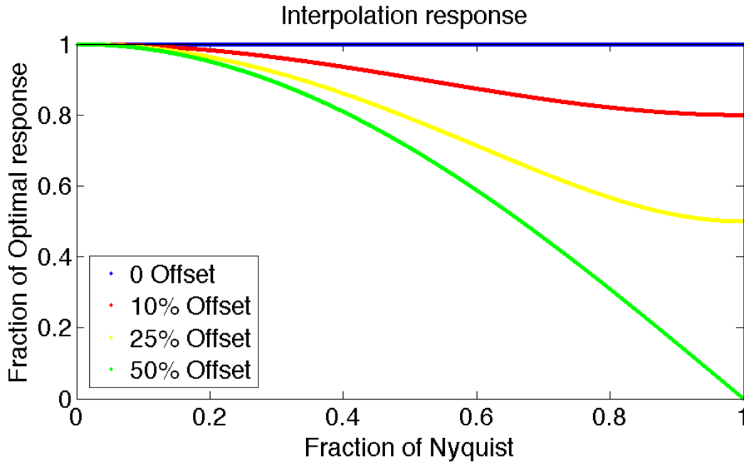
Figure 5.7: Linear interpolation response. The figure shows the loss of signal (y axis) as a function of the frequency of the signal (x axis). The four curves are the offset at which the interpolation is done. 0% refers to no interpolation and thus a 100% response. 50% is the worse case and the 0% response at Nyquist is the triangle wave case explained above.
