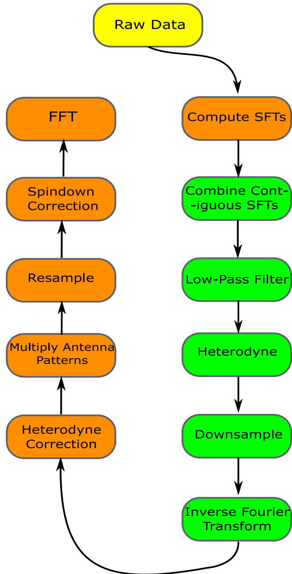
Figure 5.2: A flow-chart showing the resampling algorithm. The green refers to an operation done in the frequency domain and the orange refers to an operation done in the time domain.
