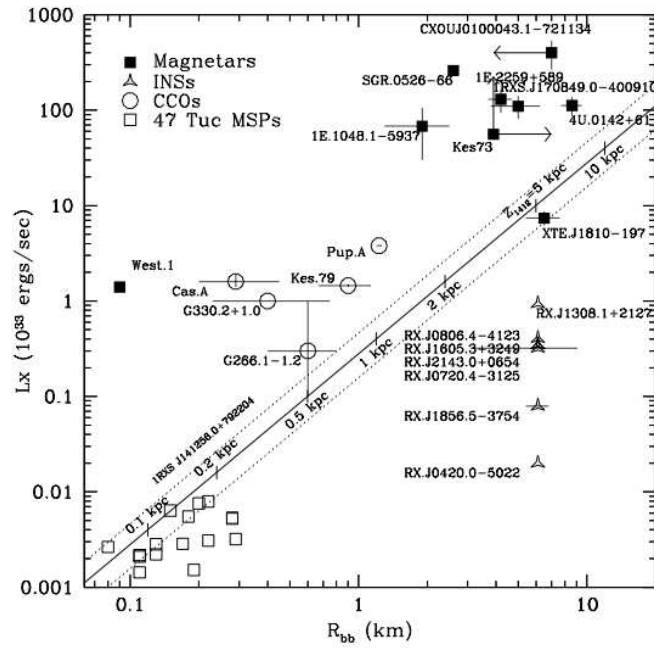
Figure 6.1: Figure reproduced with permission from [115]. Plot of blackbody radius R_{bb} and the X-Ray Luminosity L_X . Best fits for Calvera lie on the black line and the error bars are the dotted lines. All four possibilities are plotted on the same plot, so comparisons can be made with Calvera.
