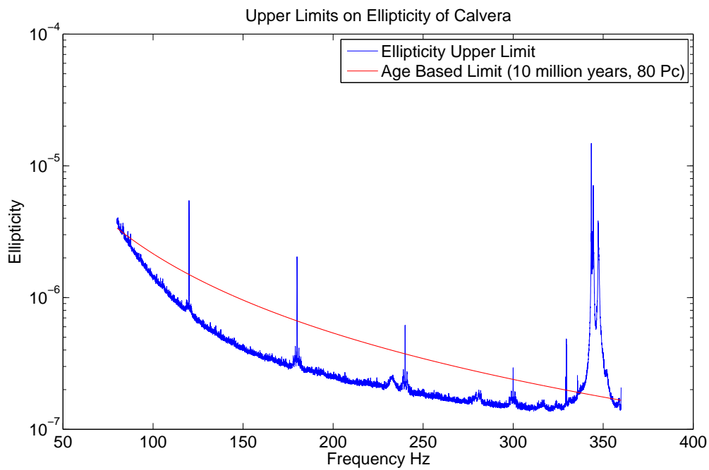
Figure 7.16: Upper limits on ellipticity of Calvera.
