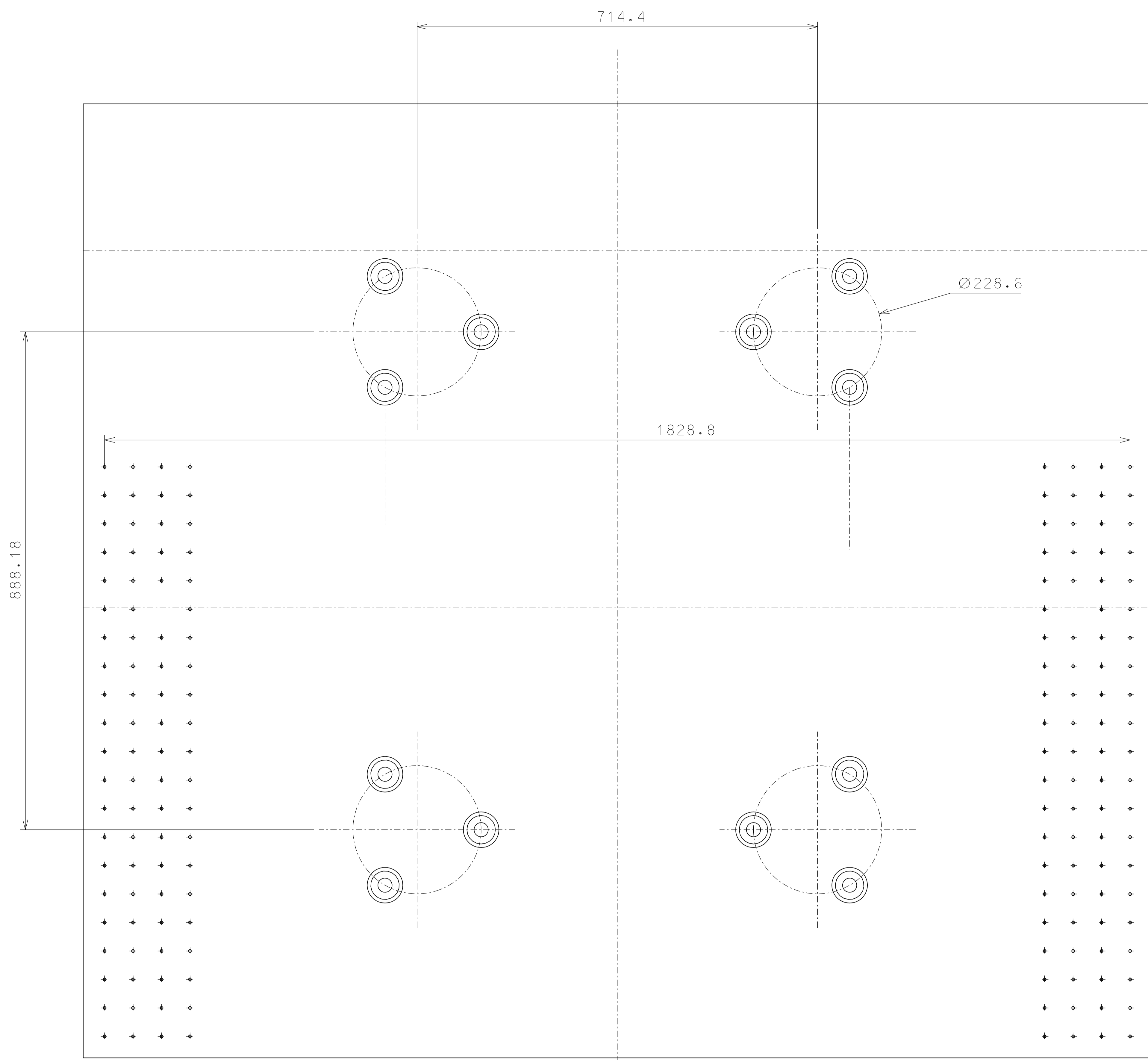
TOP VIEW
