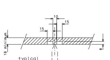
typical section D-D scale 1/2
