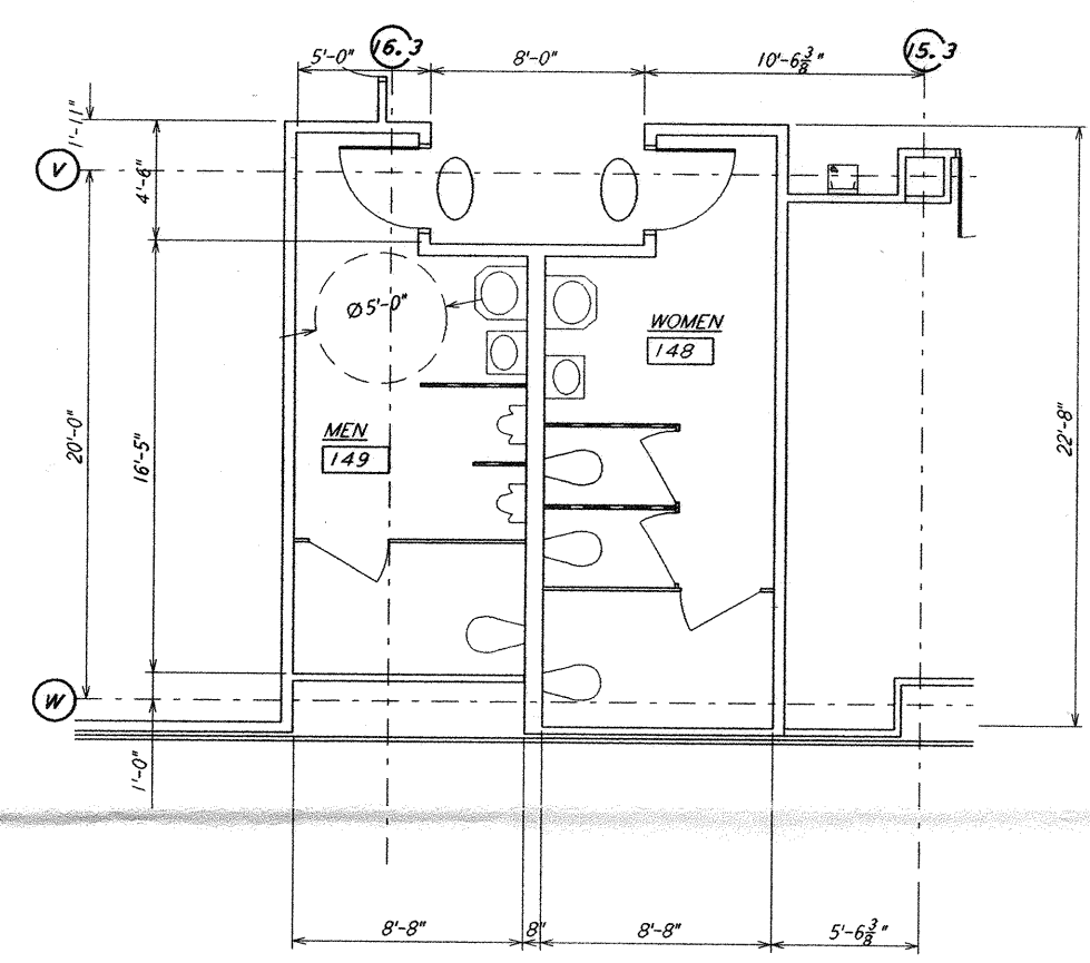
ENLARGED TOILET PLAN \frac{1}{4}'' = 1'-0'' 2 WA-A-108
