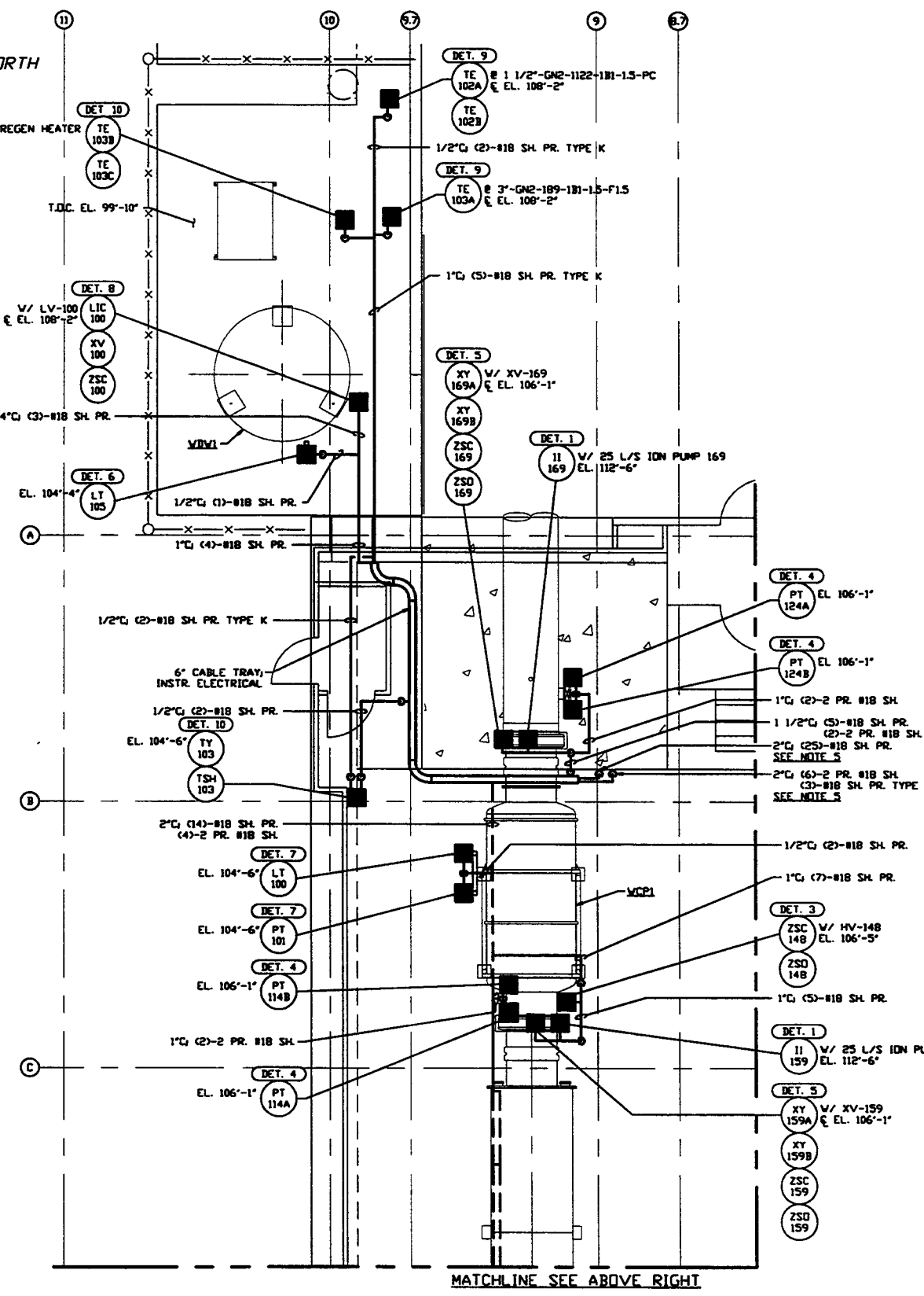
LEFT BEAM MANIFOLD PLAN @ EL. 100'-0"
