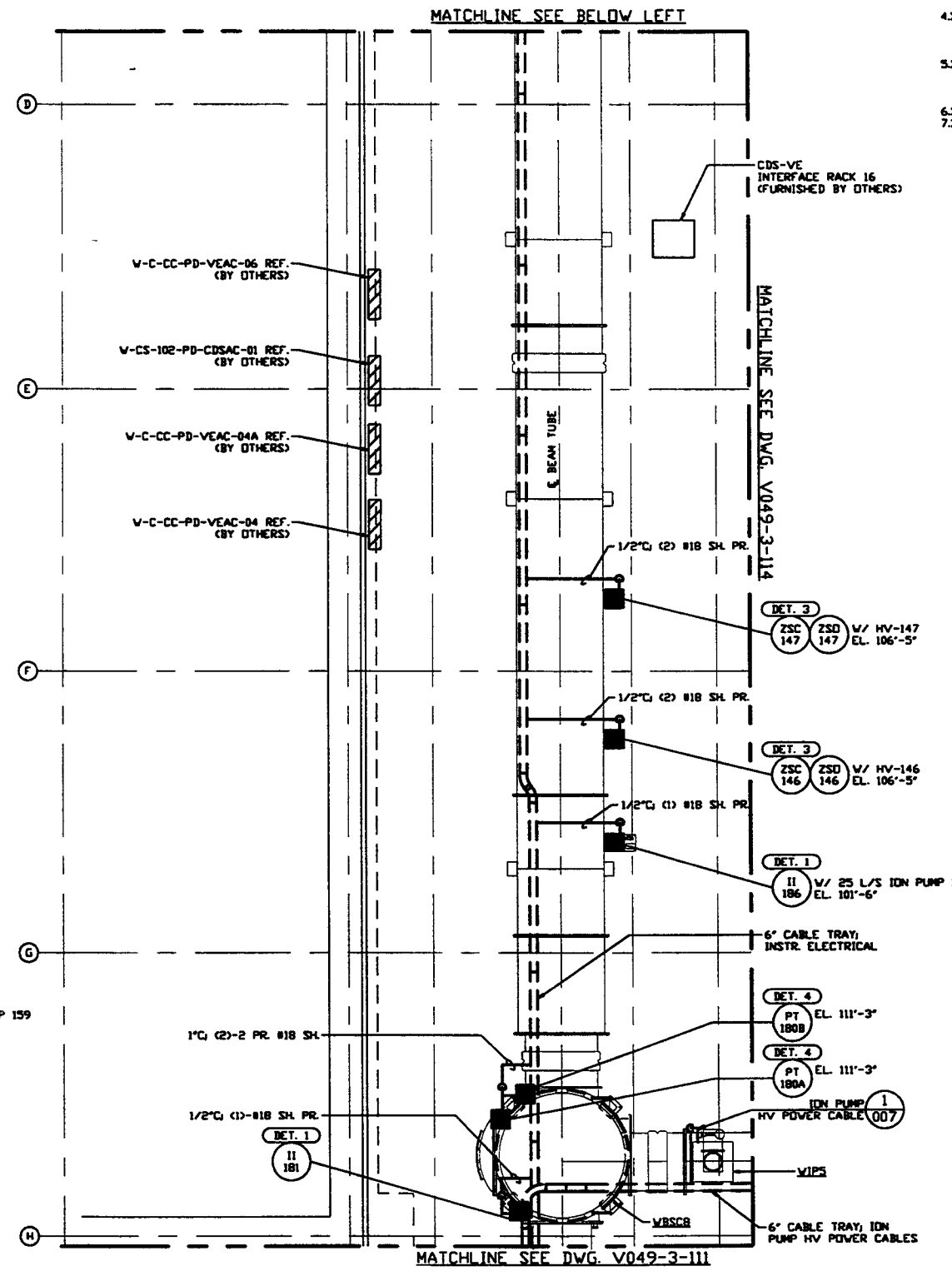
LEFT BEAM MANIFOLD PLAN @ EL. 100'-0"
