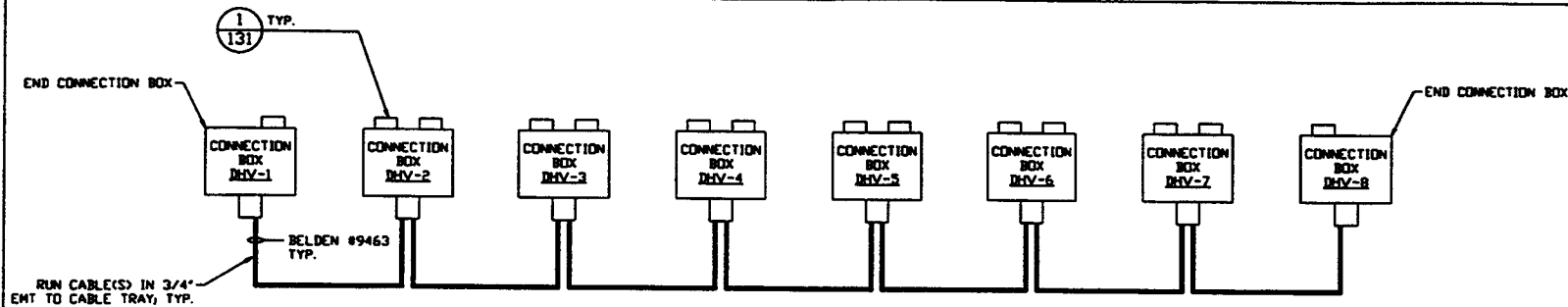
VERTEX SECTION DATA HIGHWAY INTERCONNECTION SEE PLAN FOR LOCATIONS
