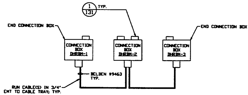
RIGHT BEAM MANIFOLD DATA HIGHWAY INTERCONNECTION SEE PLAN FOR LOCATIONS
