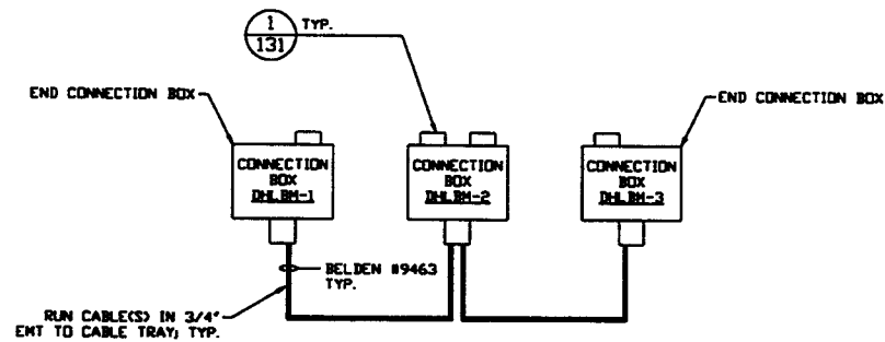
LEFT BEAM MANIFOLD DATA HIGHWAY INTERCONNECTION SEE PLAN FOR LOCATIONS
