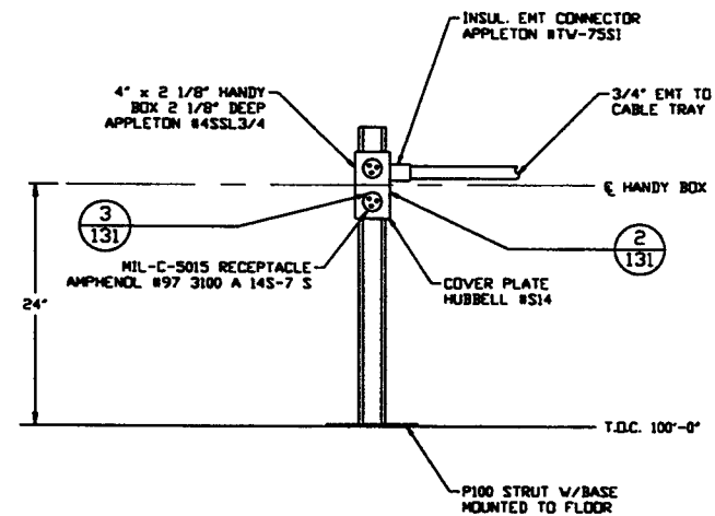
DATA HIGHWAY CONNECTION BOX MOUNTING
