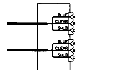
CONNECTOR WIRING OMIT WIRING FOR SECOND CONNECTOR FOR END CONNECTION BOXES
