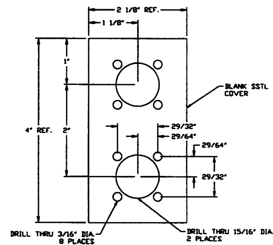
COVER PLATE DRILLING OMIT SECOND CONNECTOR HOLES FOR END CONNECTION BOXES
