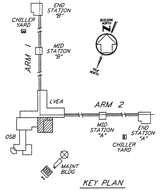
KEY PLAN 1/8" = 1'-0"
