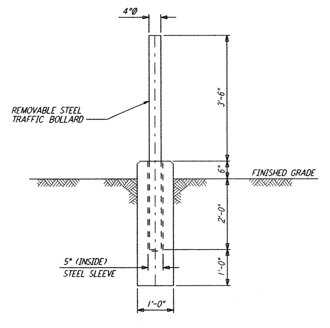
EQUIPMENT TRAFFIC PROTECTION DETAIL (4) REF LA-E-101 N.T.S.
