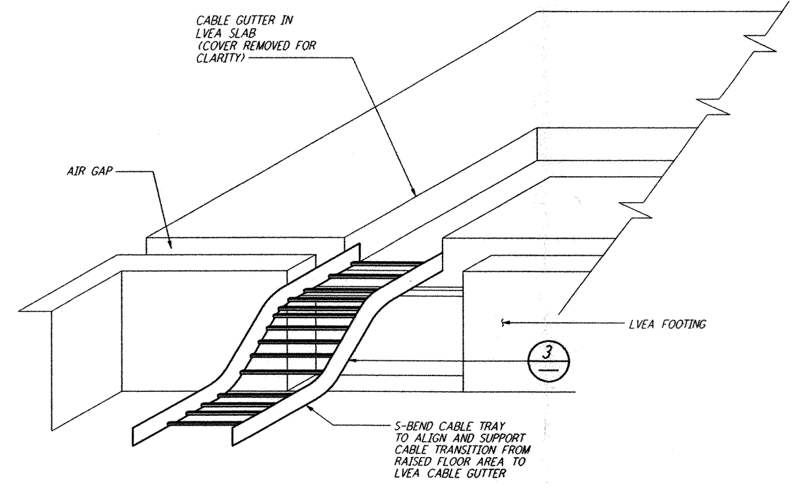
RAISED FLOOR AREA TO LVEA SLAB TRANSITION (B) REF LA-E-101 N.T.S.
