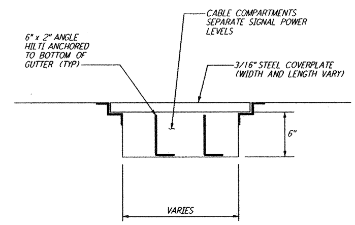
SECTION CABLE GUTTER (C) REF LA-E-101 N.T.S.
