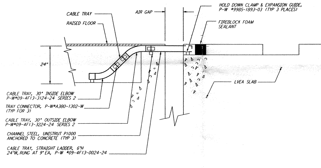
RAISED FLOOR AREA TO LVEA SLAB TRANSITION (3) REF THIS DWG N.T.S.
