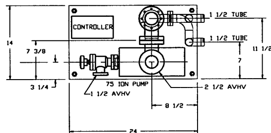
PLAN - 75 L/S ION PUMP SCALE: 1 1/2" = 1'-0"
