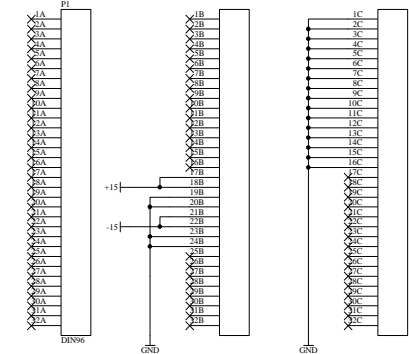
Daisy-Chained Connection to Servo Amp and Steering Mirror Modules
