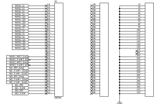
Daisy-Chained Connection to Servo Amp and Steering Mirror Modules
