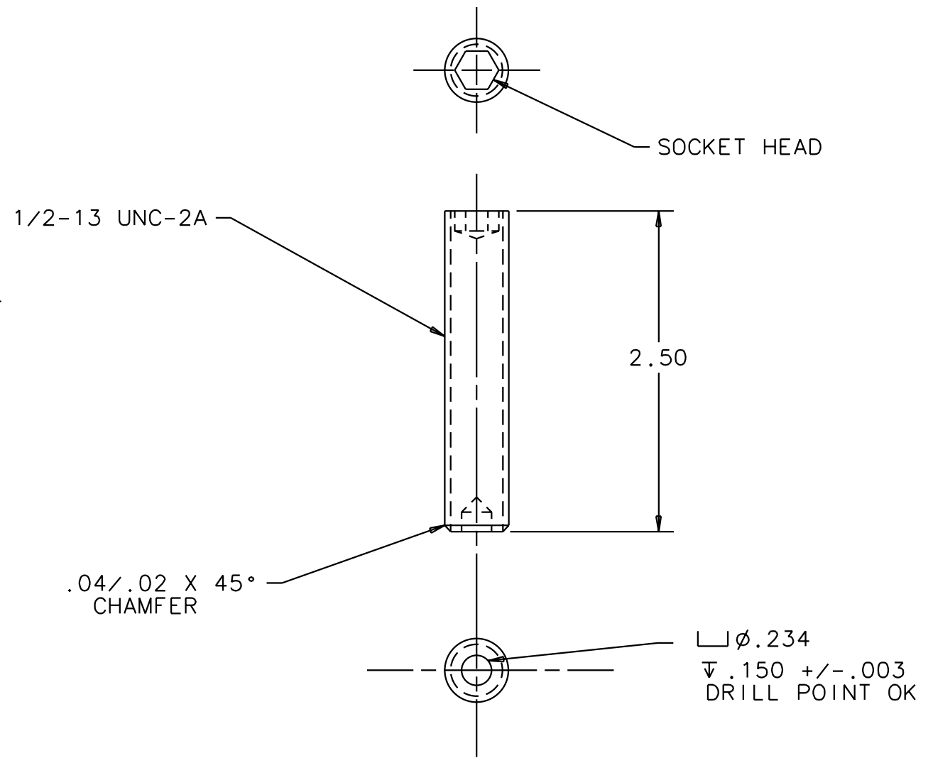
SCREW DETAIL ITEM 1
