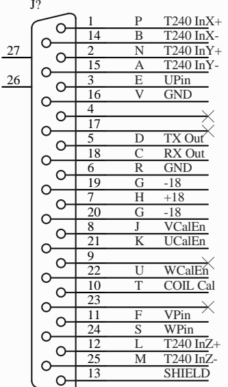
D Connector 25
