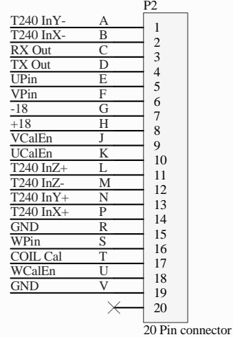
20 Pin connector
