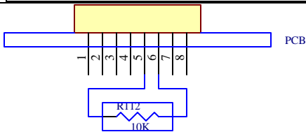
(6) New Added Resistor soldered between pin 5 and 6 on the circuit side of PCI
