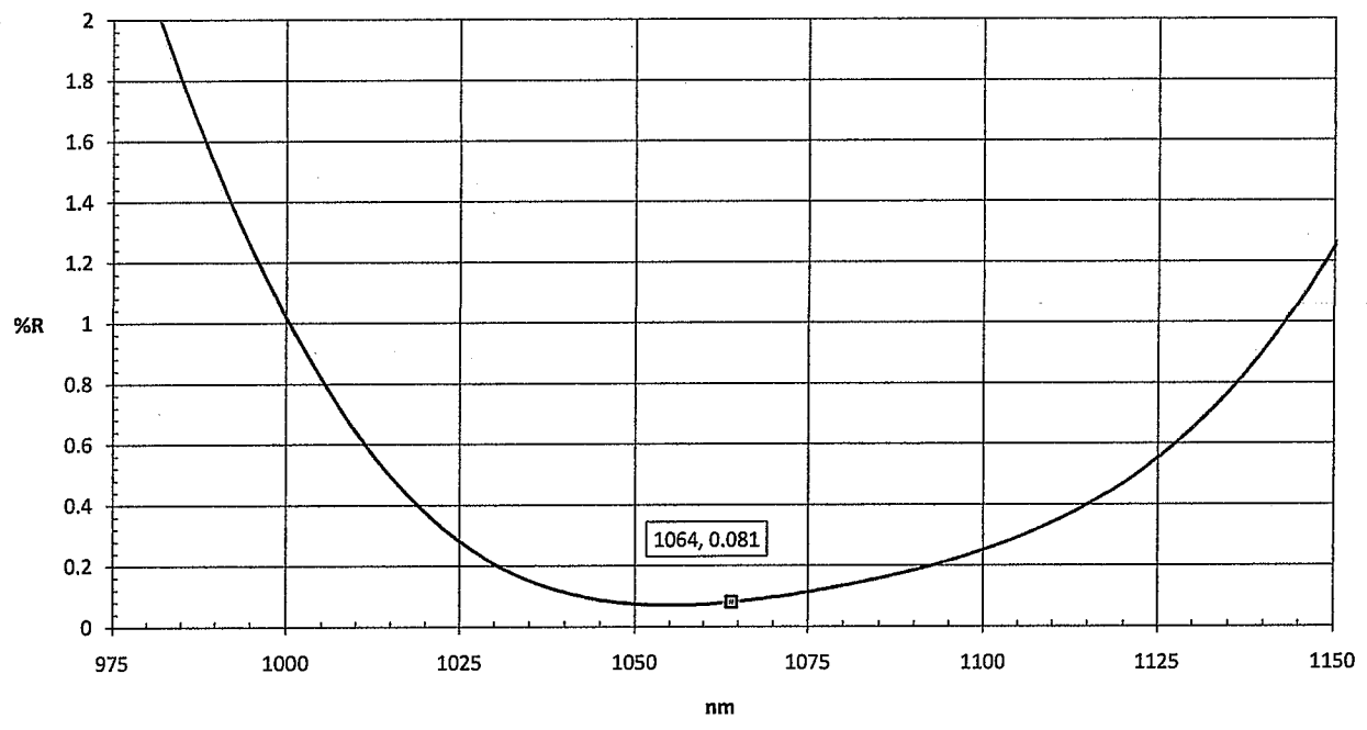
— V2-2166, FS Witness, BB, 45° P-pol, F=0.0273
