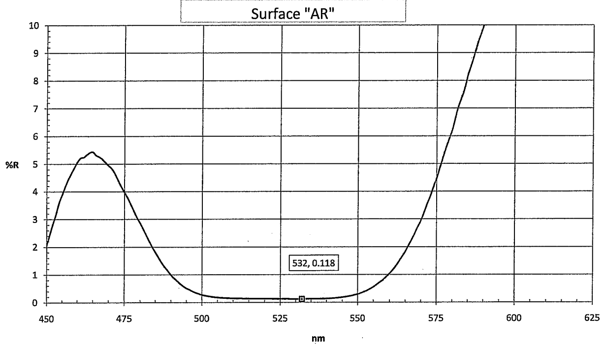
— V2-2166, FS Witness, BB, 45° S-pol, F=0.0996
