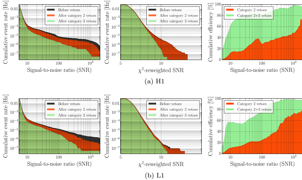
Figure 13: The effect of category 2 and jointly of category 2 and 3 vetoes on the CBC pipeline for (a) H1 and (b) L1. The left panels show the reduction in event rate as a function of SNR, the centre panels show the reduction in event rate as a function of the \chi^2 -weighted SNR, and the right panels show the cumulative efficiency as a function of SNR.
