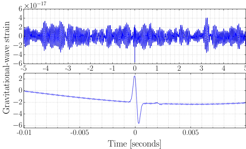
Figure 11: A spike glitch in the raw GW photodiode signal for L1. The top panel shows the glitch in context with 10s of data, while the bottom shows the glitch profile as described in the text.
