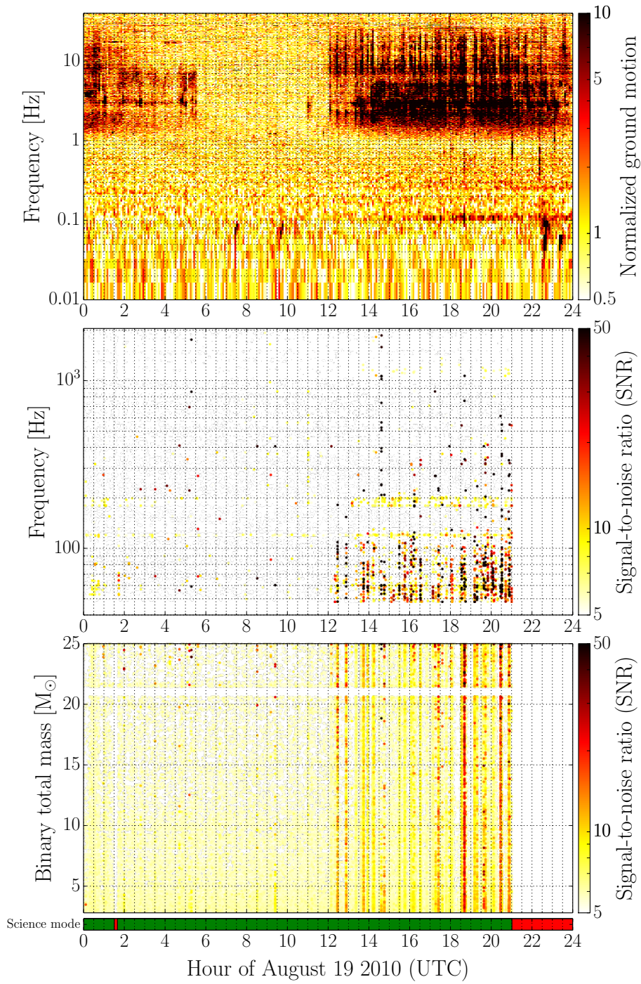
Figure 5: Seismic motion of the laboratory floor at LHO (normalized, top) and its correlation into GW burst (middle) and inspiral (bottom) analyses.
