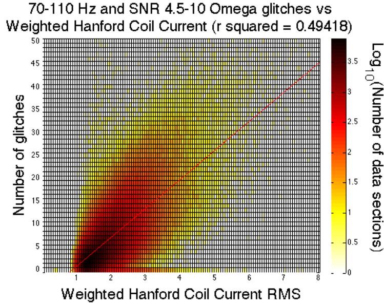
Figure 7: Correlation between low SNR glitches in the GW data, and current in the test mass coil at H1. The r^2 value measures the normalized cross-correlation through a least-squares fit. This correlation is indicative of the Barkhausen effect.
