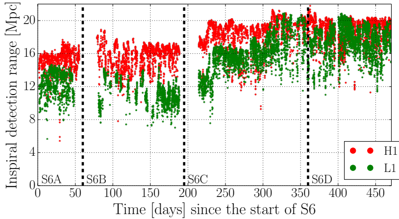
Figure 4: The inspiral detection range of the LIGO detectors throughout S6 to a binary neutron star merger, averaged over sky location and orientation. The rapid improvements between epochs can be attributed to hardware and control changes implemented during commissioning periods.
