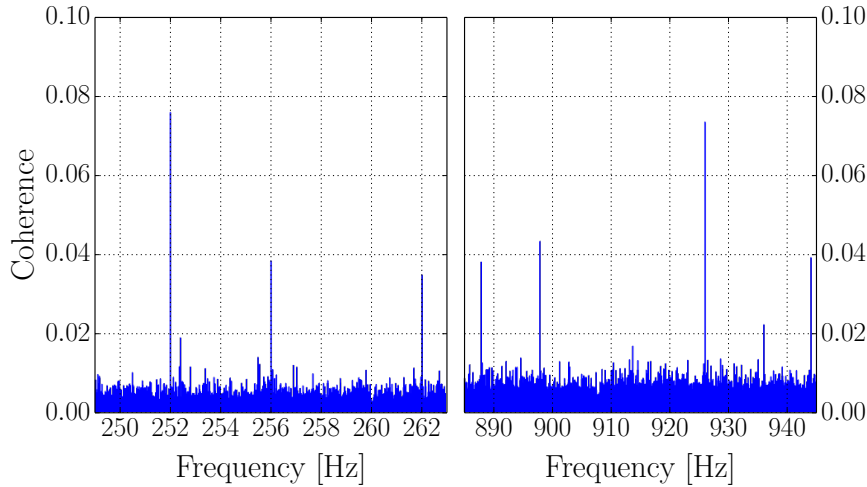
Figure 10: The coherence between the L1 GW readout signal and data from a magnetometer in the central building at LLO over one week of March 2010. 2 Hz and 16 Hz harmonics were seen to be coherent at numerous locations across the operating band of both interferometers, affecting the sensitivity of long-duration GW searches.
