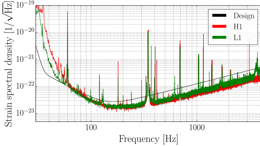
Figure 3: Typical strain amplitude sensitivity of the LIGO detectors during S6.
