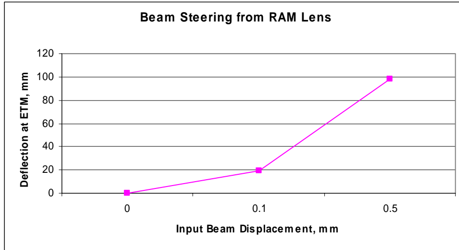
Figure 40: Beam Steering by RAM Lens
