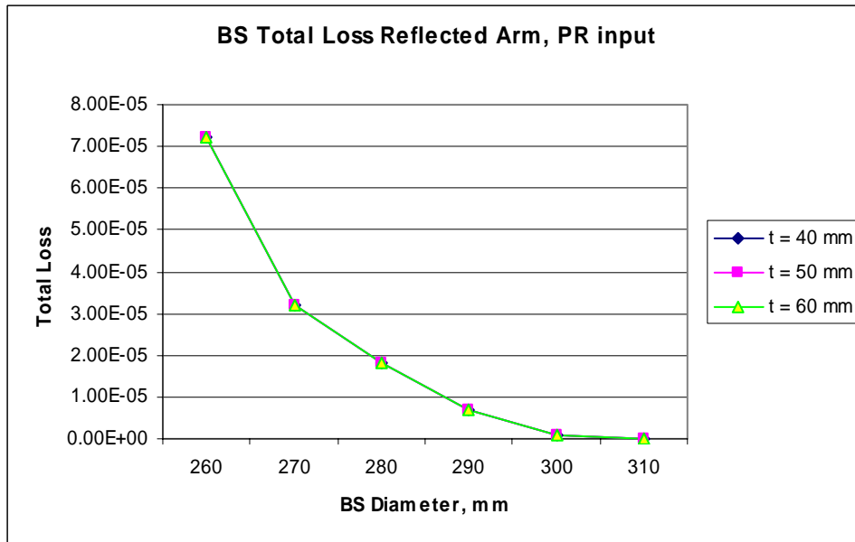
Figure 35: BS Total Loss Reflected arm, PR Input
