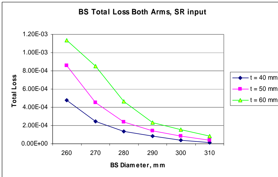
Figure 39: BS Total Loss Both Arms, SR Input
