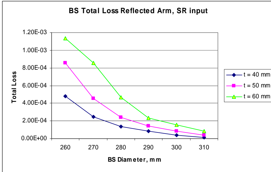
Figure 38: BS Total Loss Reflected Arm, SR Input
