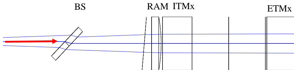
Figure 33: Optical Schematic, Alternative Design with Lens in RAM
