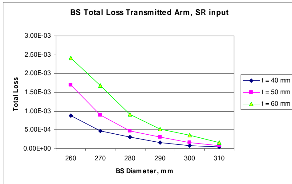
Figure 37: BS Total Loss Transmitted Arm, SR Input
