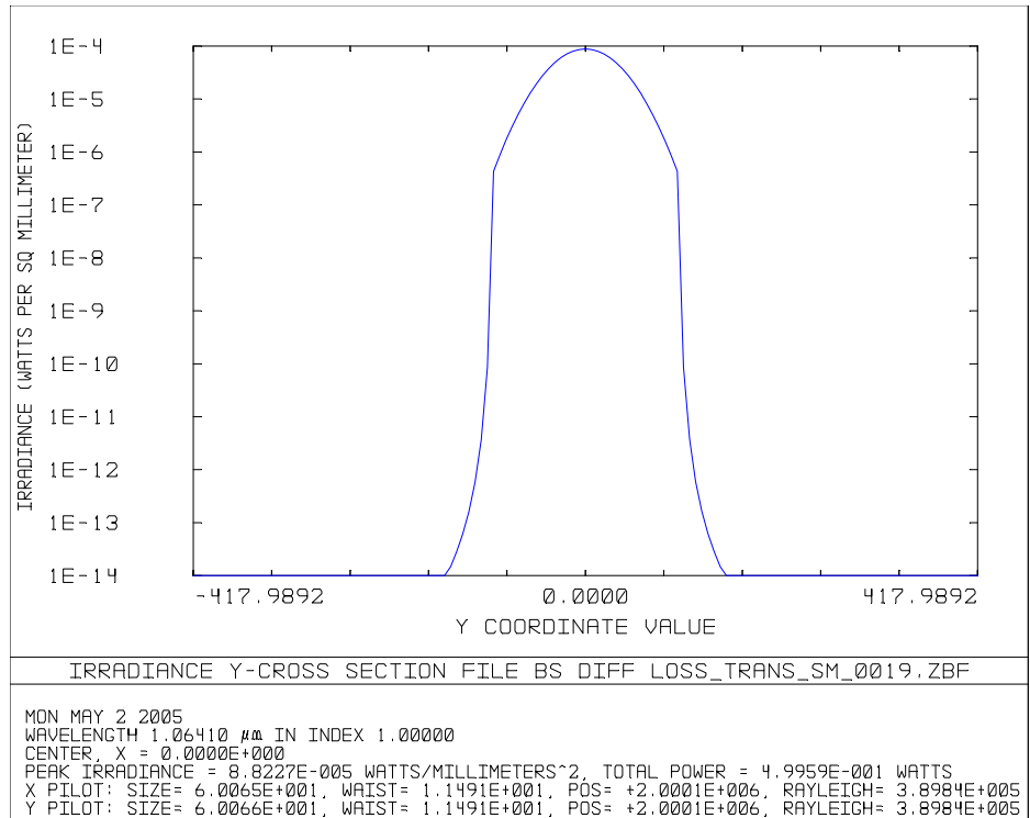
Figure 17: Y-cross Section at ITMx HR, SR Input, Transmitted Arm
