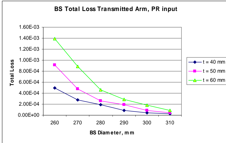
Figure 34: BS Total Loss Transmitted arm, PR Input
