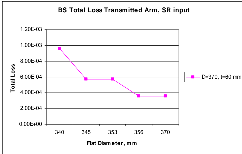
Figure 31: Power Loss in Transmitted Arm, SR Input from Flats
