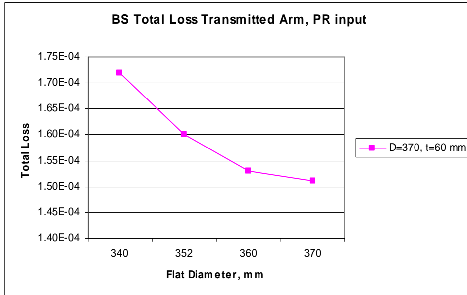
Figure 32: Power Loss in Transmitted Arm, PR Input from Flats
