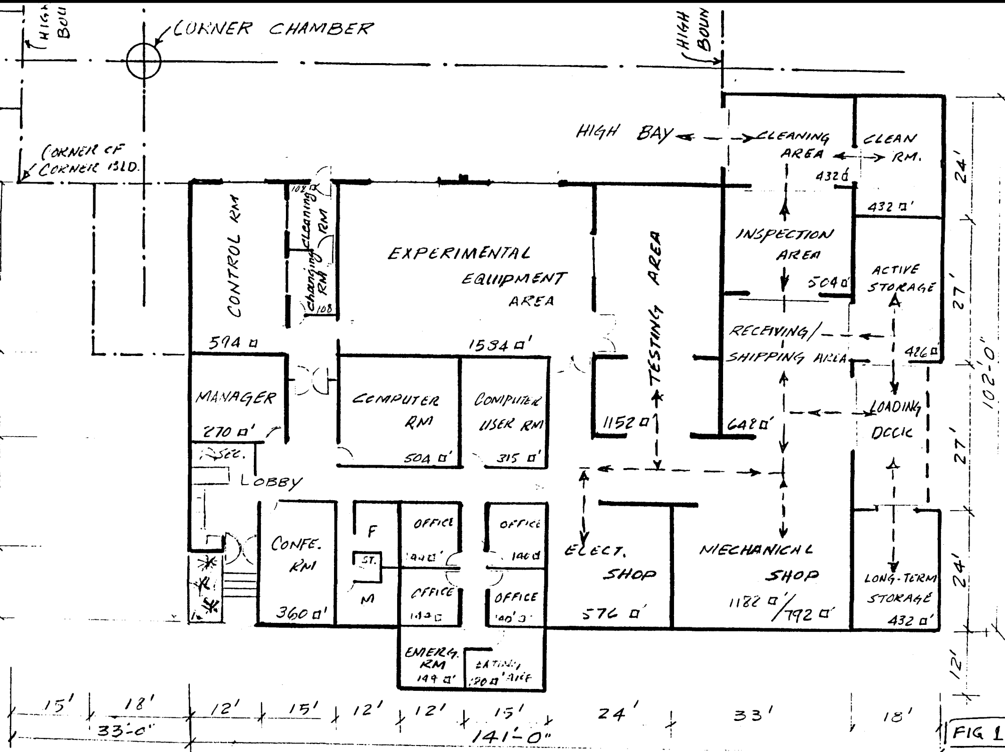
FLOOR PLAN OF OFFICES & SHOPS
