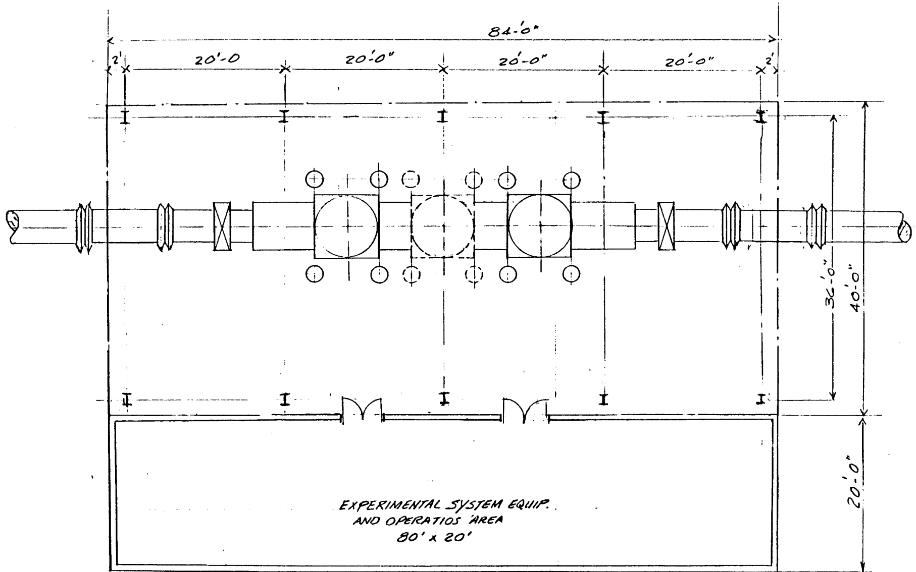
FLOOR PLAN OF MID-STATION SCALE \frac{1}{8}'' = 1'-0''
