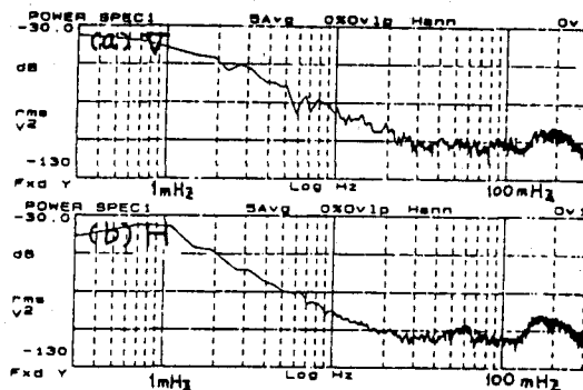
Fig. 3 Power spectra for (a) vertical and (b) horizontal seismic motions measured on the floor in the Tsukuba straight section.
