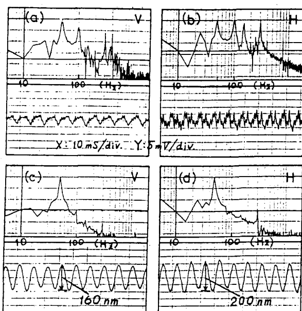
Fig. 2 Seismic motion measured (a,b) on the base for the QC1 magnet and (c,d) on the back of the QC1 magnet. Figs (a,c) show the vertical motion, and (b,d) the horizontal motion respectively. In each figure the top graph shows the power spectrum and the bottom graph shows the output from measuring heads.
