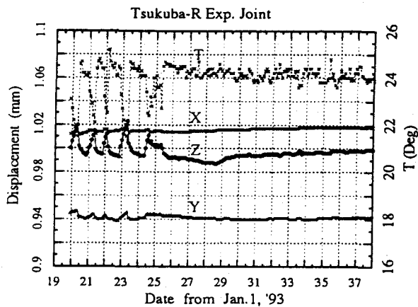
Fig.10 Relative displacement of the floor at the expansion joint in Tsukuba straight section.
