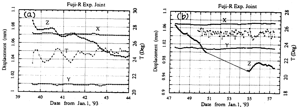
Fig.11 Relative displacement of the floor at the expansion joint in Fuji straight section during the period (a) Feb.8 - 12 and (b) Feb.16 - 26, 1993.
