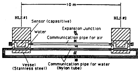
Fig. 6 Hydrostatic Leveling System.
