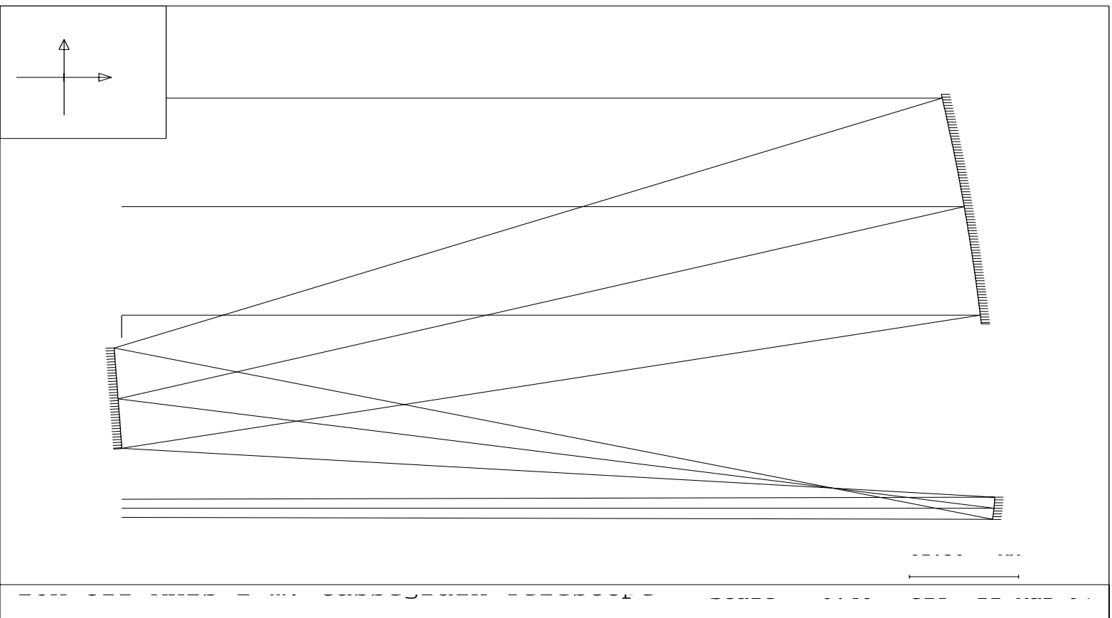
Figure 12: PO Beam Reducing Telescope
