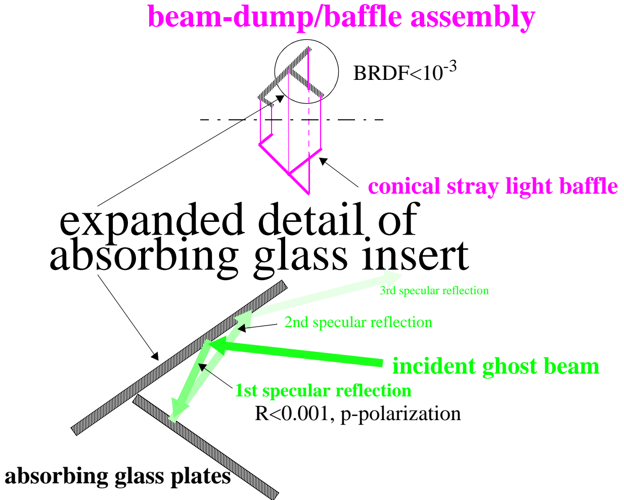
Figure 11: Beam-dump/baffle Concept
