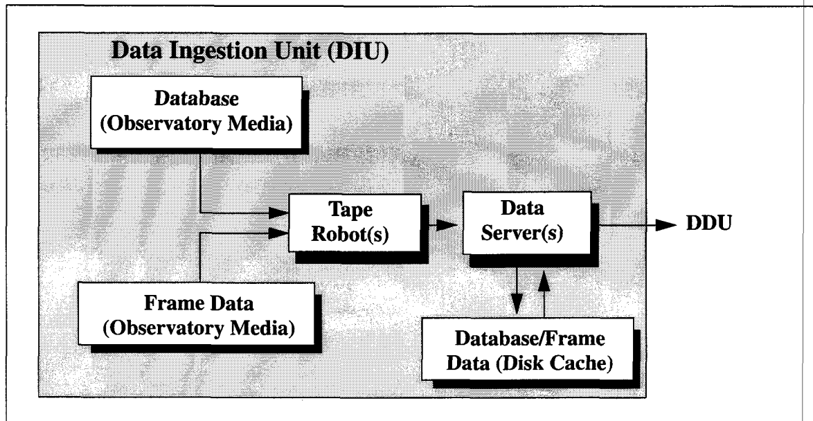
Figure 12 Data Ingestion (DIU) Block Diagram
