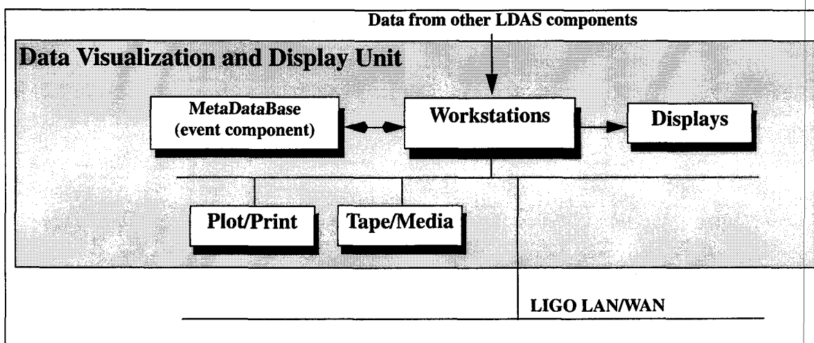
Figure 17 DVU Block Diagram
