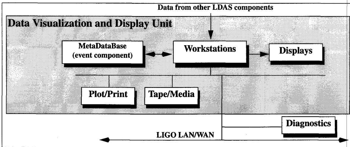
Figure 11 DVU Block Diagram
