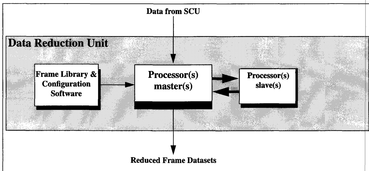
Figure 15 Data Reduction Unit Block Diagram
