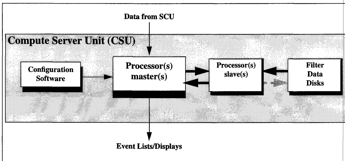
Figure 10 Compute Server Unit Block Diagram
