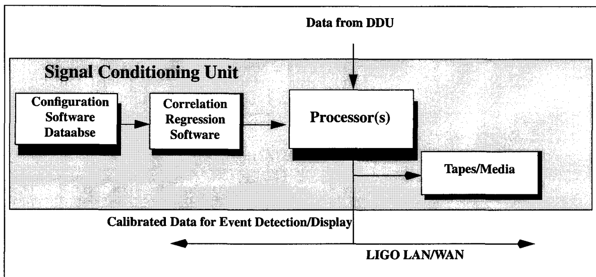
Figure 9 Signal Conditioning Block Diagram
