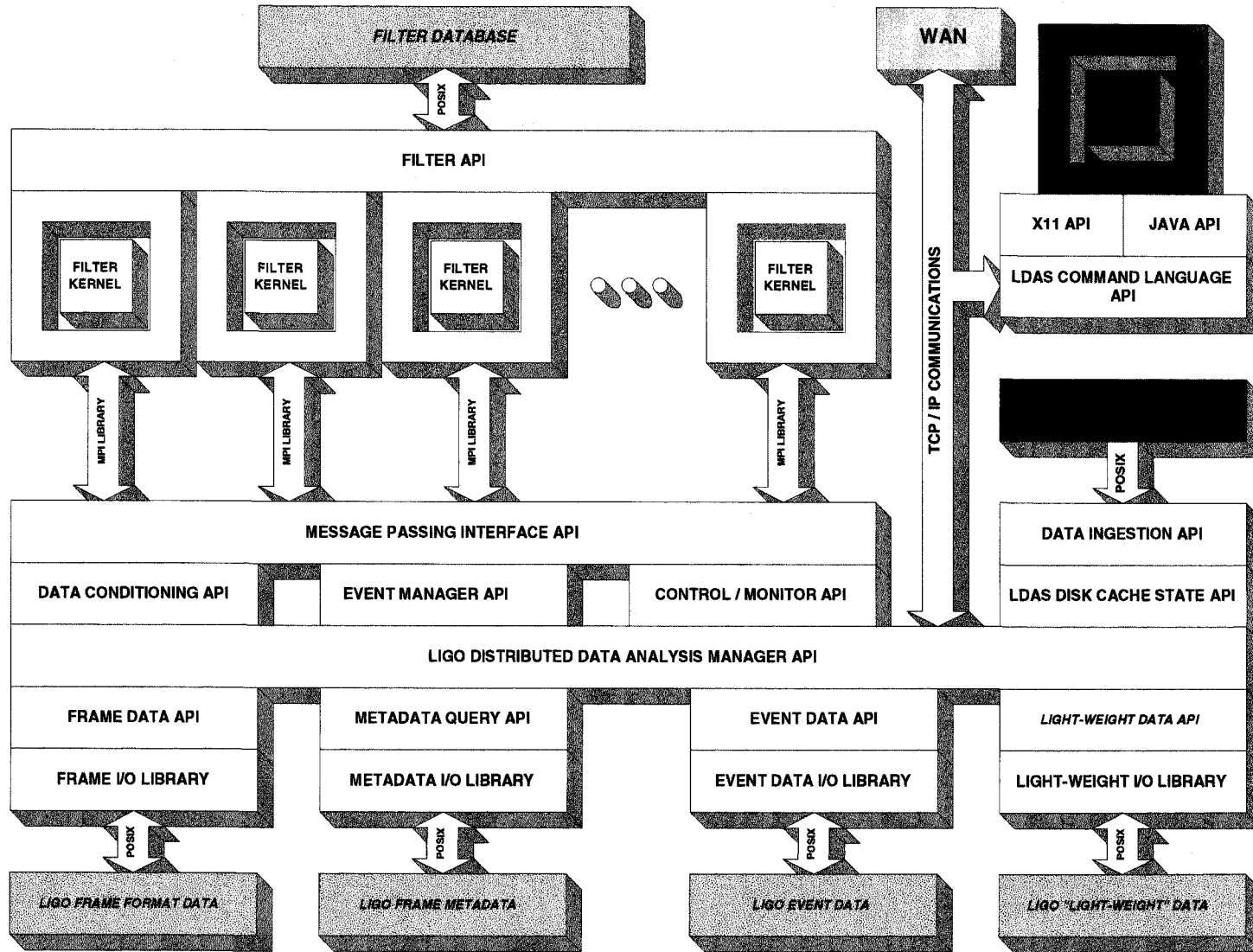
Figure 7 Block Diagram of the LDAS Software Components
