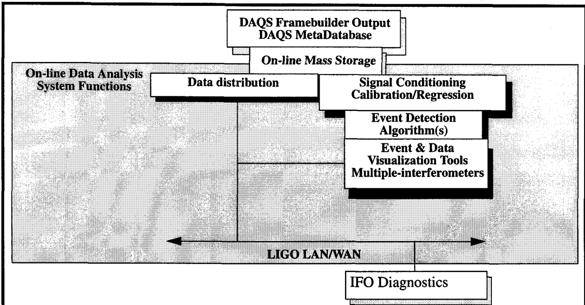
Figure 2 LDAS Functional Block Diagram - On-line Analysis
