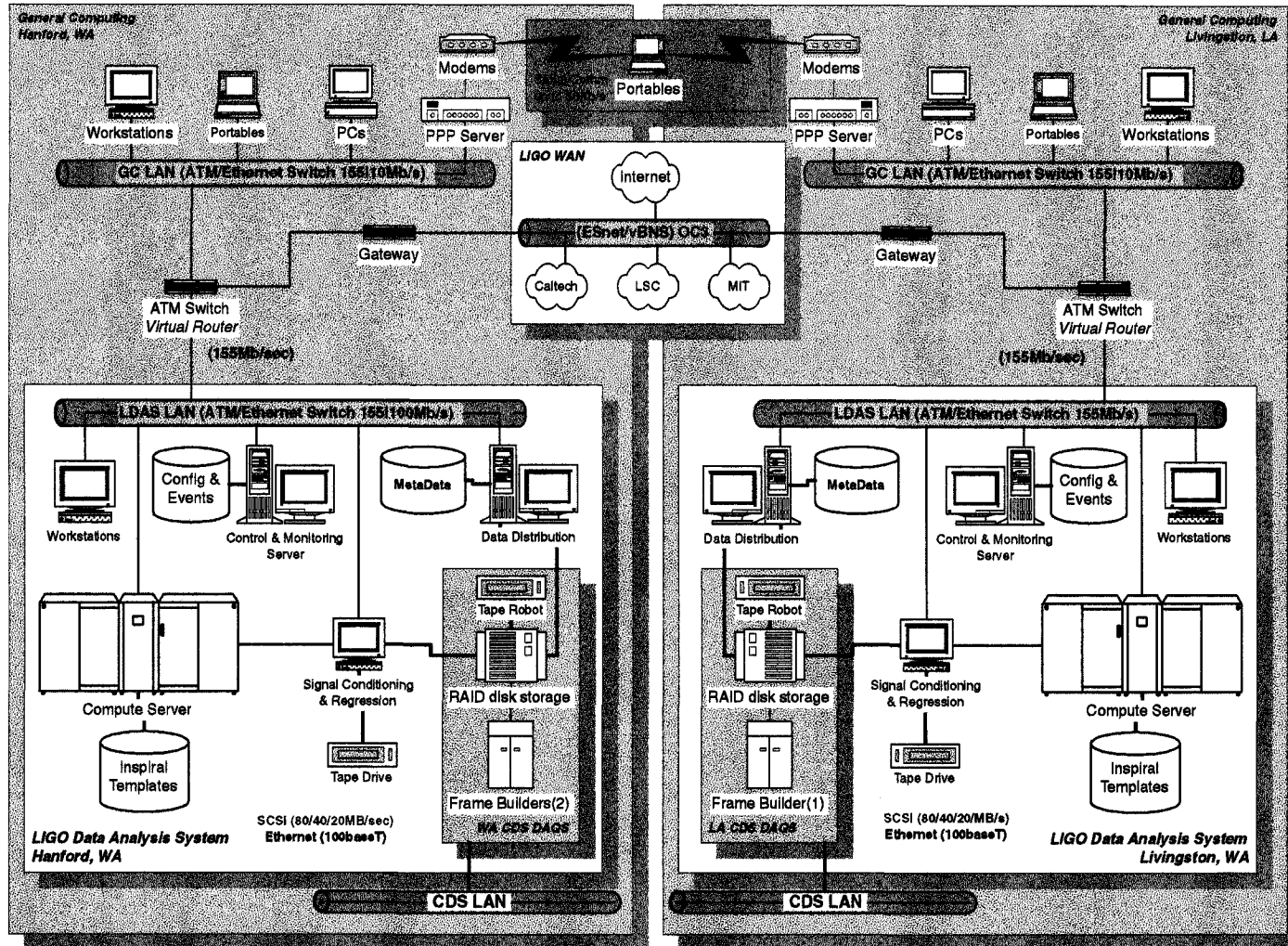
Figure 4 LDAS architecture for the on-line component
