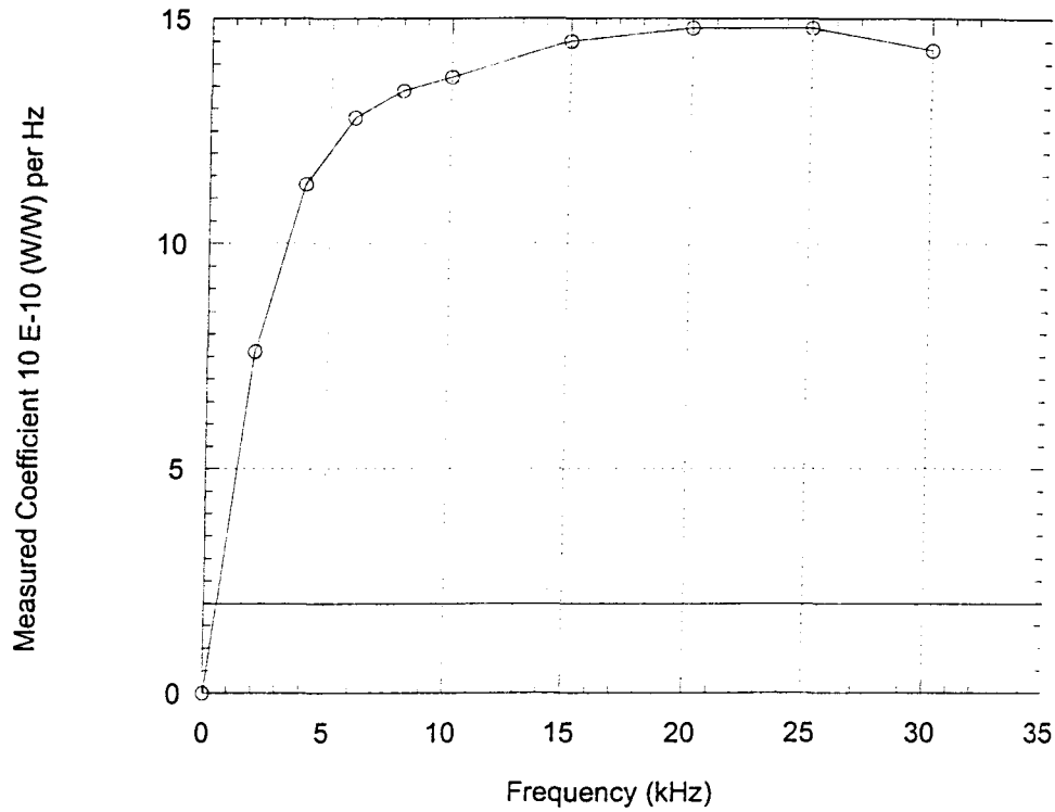
Fig. 3. Measured fractional power change (W/W) per Hz of frequency change. The straight line shows the coefficient defined in specification 19 of LIGO-E970055-02-D.
