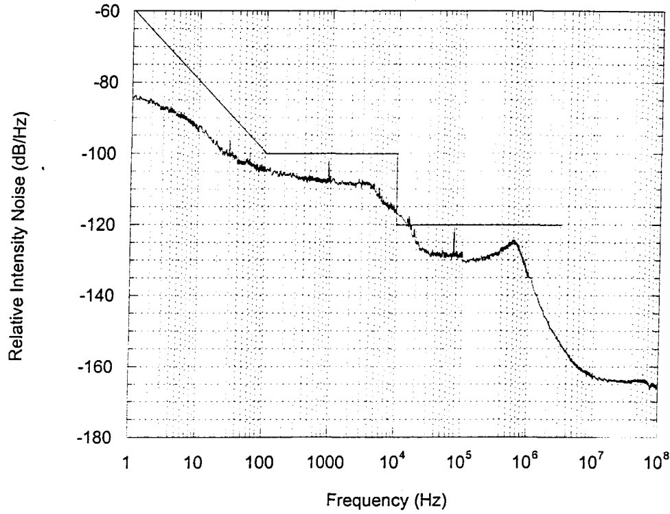
Fig. 1. Measured relative intensity noise of the amplified output at 10 mA photodetected current. The straight line shows specification 6, 7 and 8 of LIGO-E970055-02-D.
