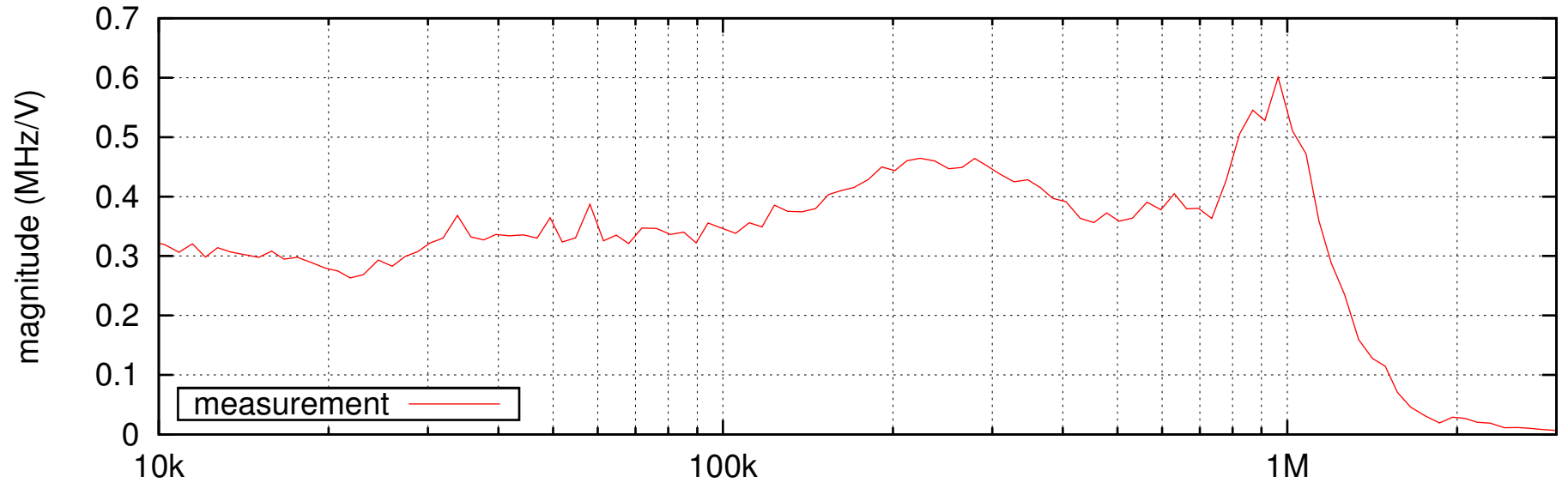
Transfer function from VCO modulation input to laser frequency
