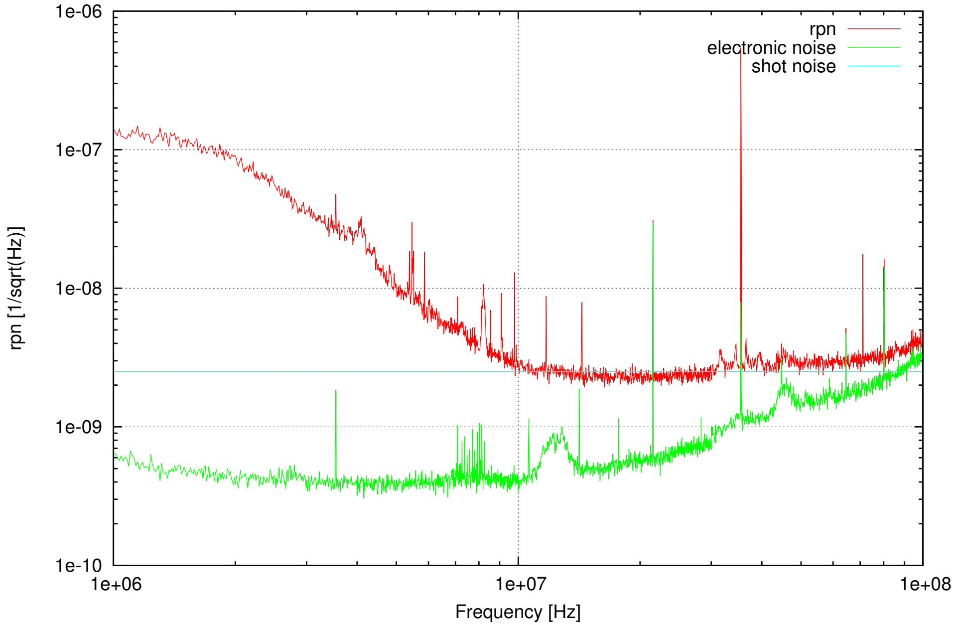
200W laser relative power noise at high frequencies
