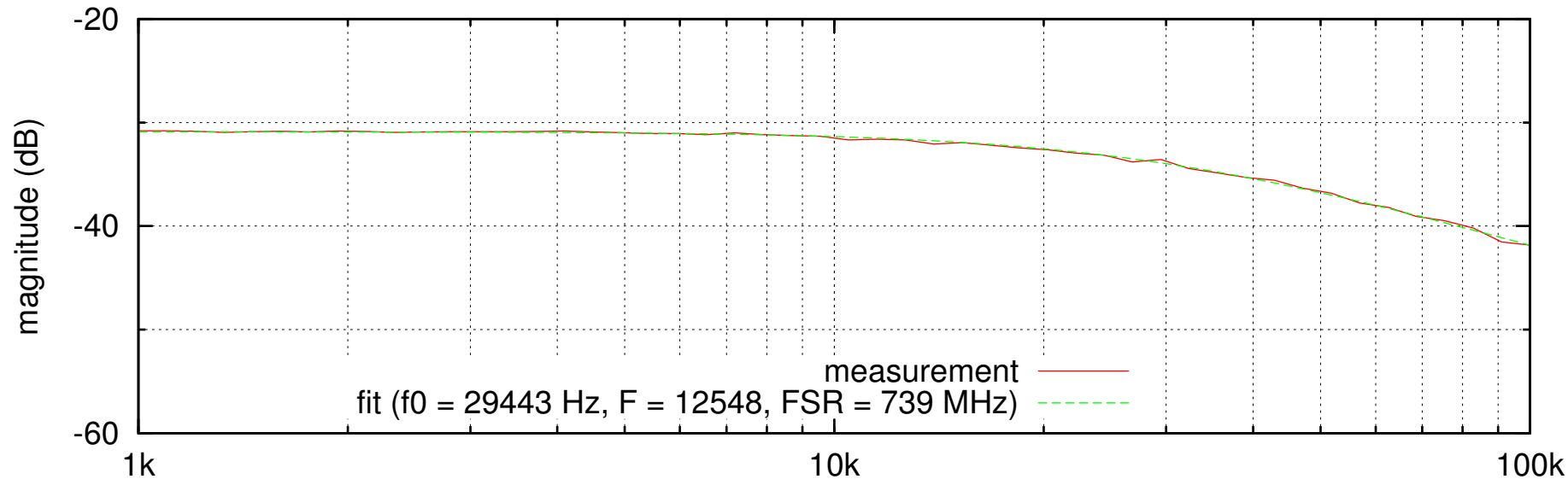
Power modulation transfer function from upstream to downstream of the reference cavity
