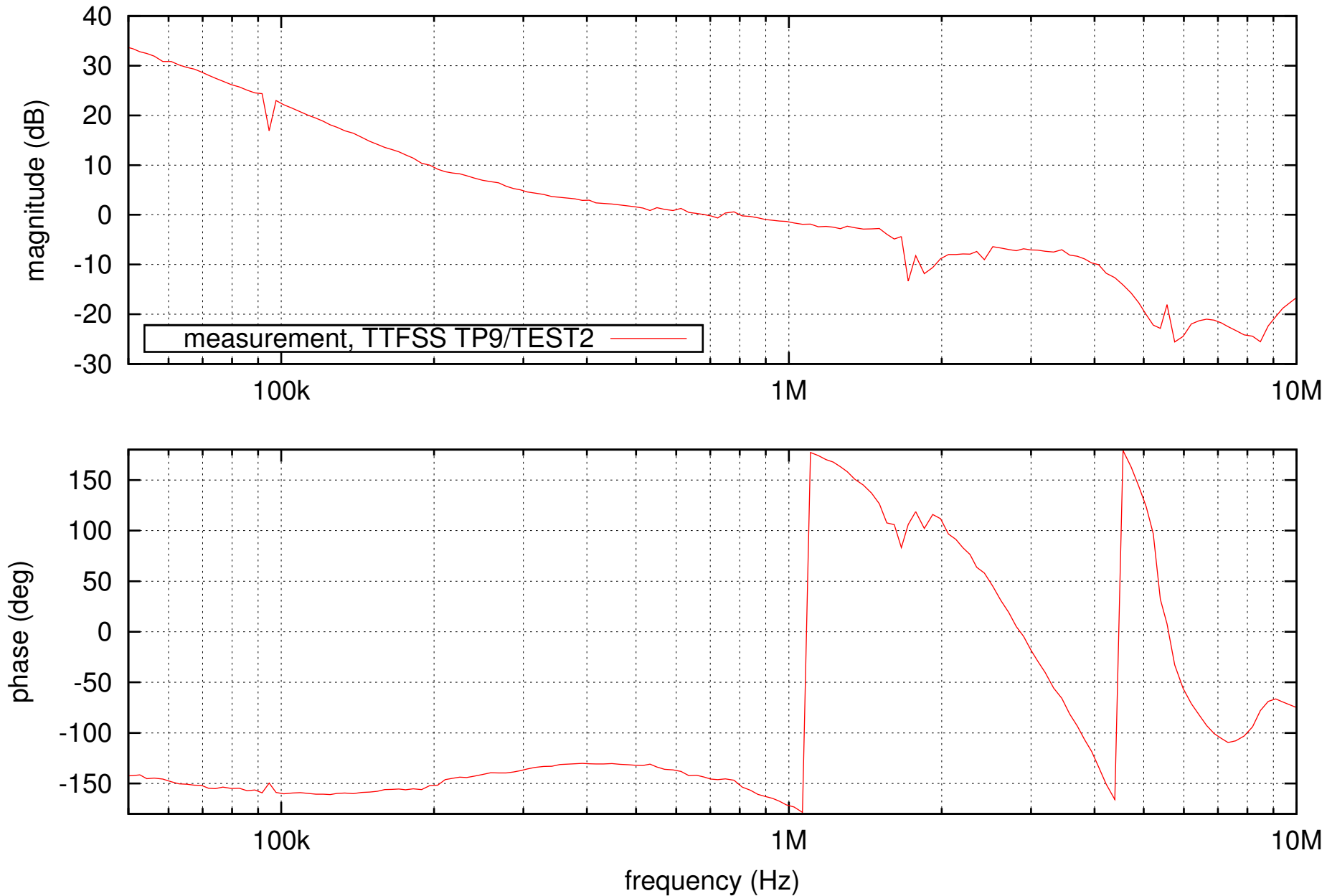
Transfer function of TTFSS (after modifications)
