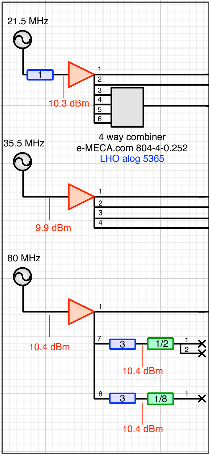
Remote Rack C3
