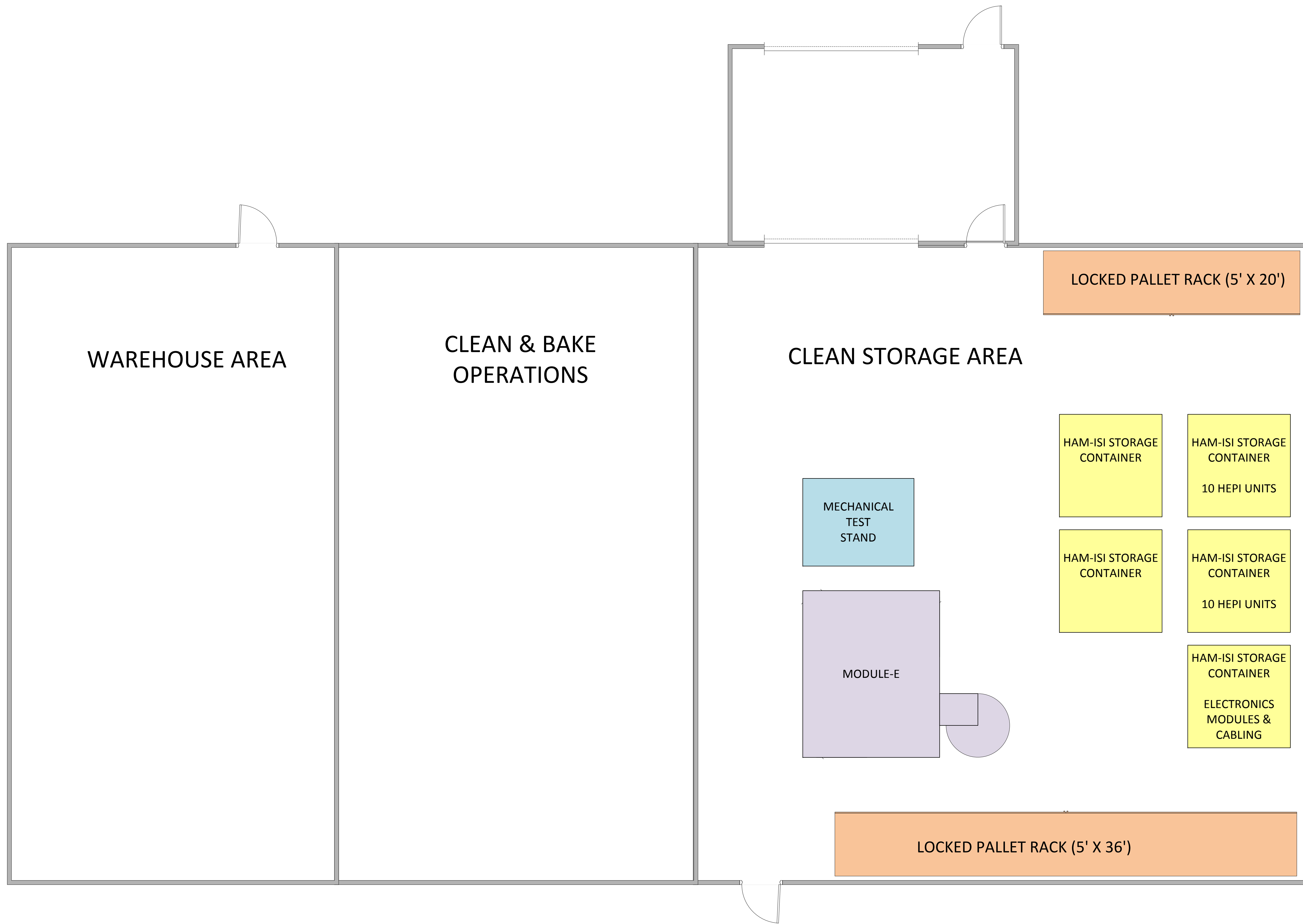
D1300035-v1 LTS VPW LAYOUT, WASHINGTON - PLAN VIEW
