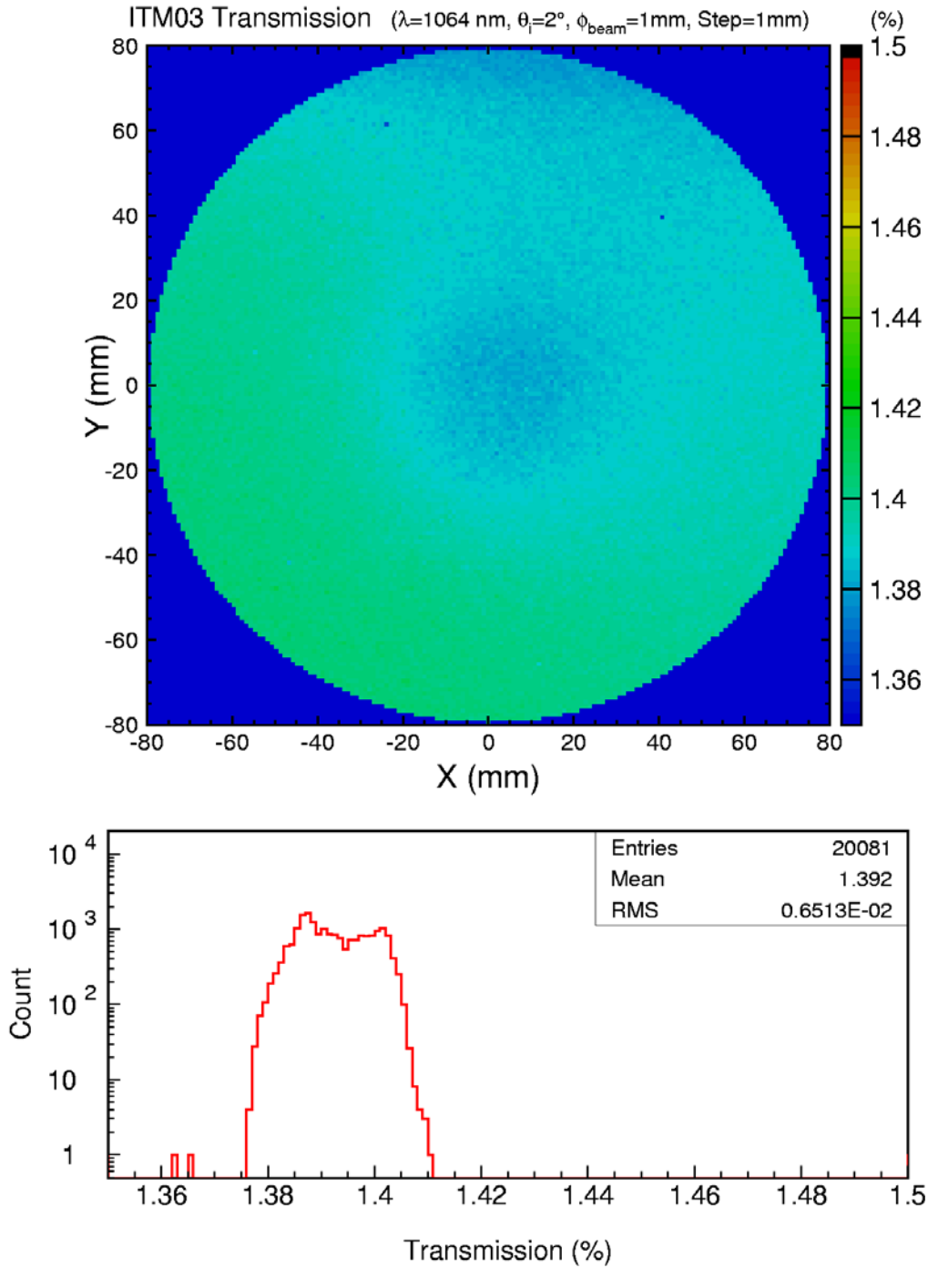
Fig. 1 ITM03 transmission over a 160 mm diameter aperture.
