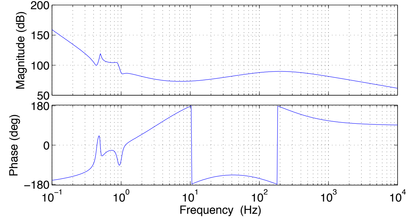
DARM Sensing
